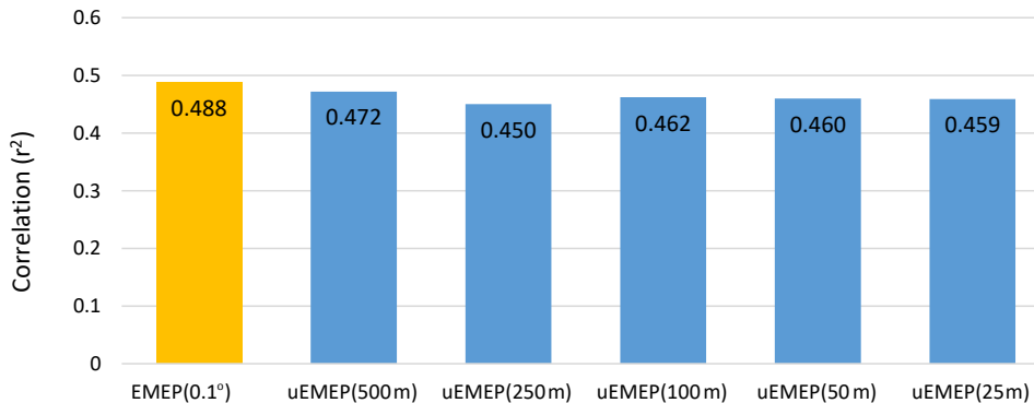
PM 2.5 r 2 due to changes in uEMEP grid resolution
