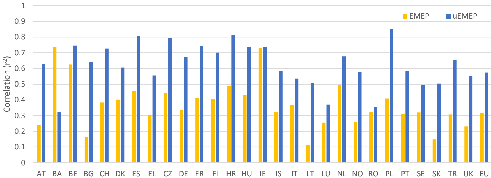
Spatial correlation ( r^2 ) NO 2 per country
