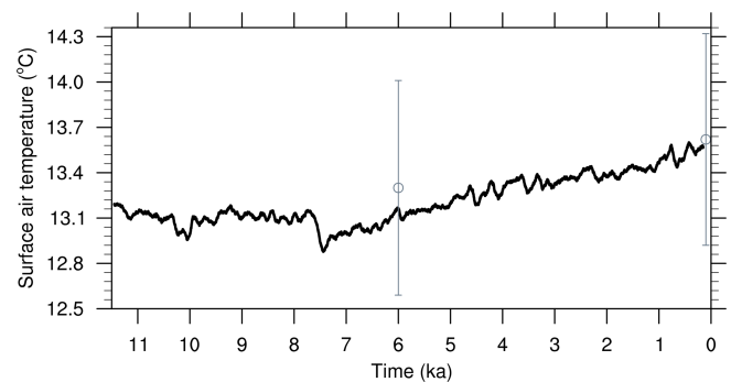
Figure 4. Global annual mean surface air temperature since 11.5 ka under the all-forcing simulation. The time series is smoothed by a 101-year moving average. The gray circles at 6 and 0.1 ka stand for the Middle Holocene and preindustrial results simulated by the arithmetic mean of the 14 PMIP4 models, with gray vertical error bars representing plus and minus 1 standard deviation for 14 models.
