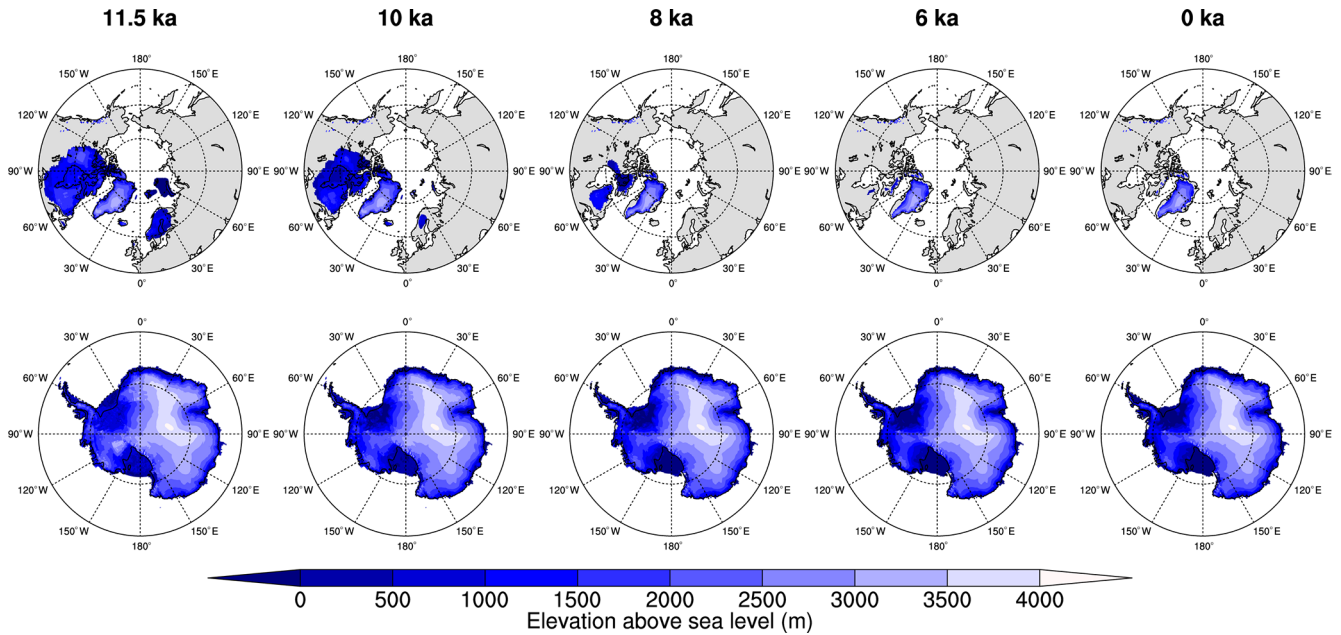
Figure 3. Northern Hemisphere (top) and Southern Hemisphere (bottom) ice sheet elevation at 11.5, 10, 8, 6, and 0 ka (1950) for the ICE-6G_C reconstruction at 10 arcmin horizontal resolution; elevation is plotted where the fractional ice mask is more than 0.5 (Peltier et al., 2015).
