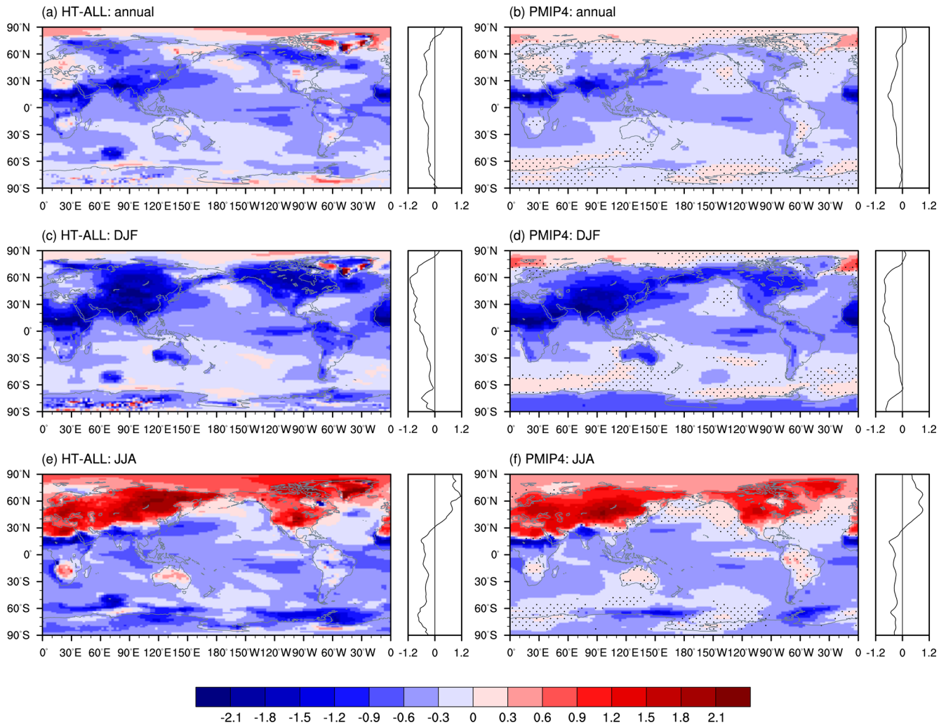
Figure 6. Changes in (a, b) annual, (c, d) DJF, and (e, f) JJA mean surface air temperatures (units in °C) (a, c, e) between the averages for 6 \text{ ka} \pm 0.05 \text{ ka} and the last 101 years (i.e., 1750–1850) in the HT-ALL simulation and (b, d, f) between the Middle Holocene and preindustrial simulations in the arithmetic mean of the 14 PMIP4 models, as listed in Fig. 5. The zonal mean changes are shown on the right of each panel. The dotted areas in (b), (d), and (f) represent less than 70 % of the PMIP4 models agree with the sign of multimodel mean change.
