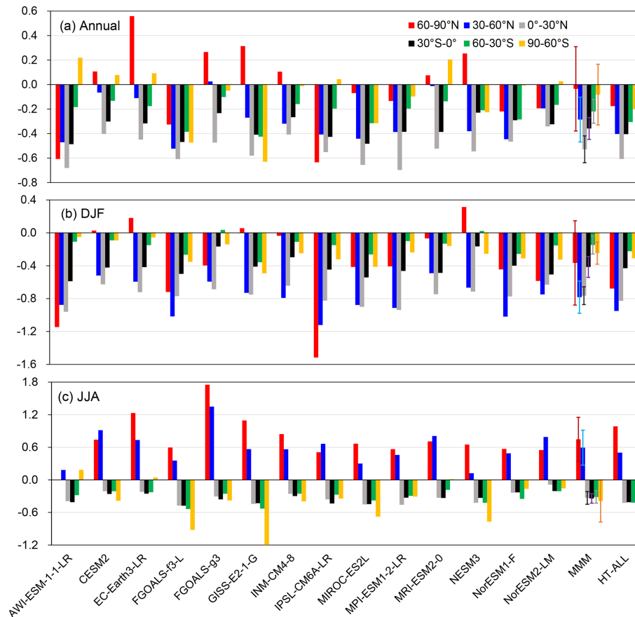
Figure 7. Zonal averaged changes in (a) annual, (b) DJF, and (c) JJA mean surface air temperatures (units in °C) between the Middle Holocene and preindustrial simulations in the 14 PMIP4 models and their arithmetic mean (MMM), as well as between the averages for 6 ka \pm 0.05 ka and the last 101 years (i.e., 1750–1850) in the HT-ALL simulation. Red, blue, gray, black, green, and orange bars represent the changes averaged over the zonal bands of 60–90° N, 30–60° N, 0°–30° N, 30° S–0°, 60–30° S, and 90–60° S, respectively. The error bar for the multimodel mean change represents plus and minus 1 standard deviation for the 14 PMIP4 models.
