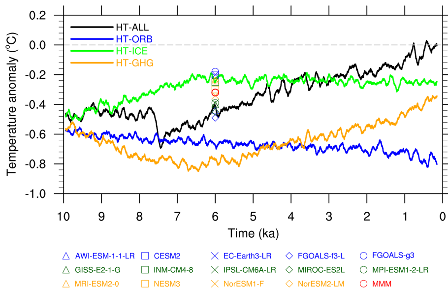
Figure 5. Global annual mean surface air temperature anomaly since 10 ka under the all-forcing (HT-ALL – black) and the single-forcing (HT-ORB – blue; HT-ICE – green; HT-GHG – orange) simulations relative to the last 101 years of the all-forcing simulation. All of the time series are smoothed by a 101-year moving average. The triangle, square, cross, diamond, and circle symbols at 6 ka stand for the Middle Holocene minus preindustrial results simulated by the 14 PMIP4 models and their multimodel arithmetic mean (MMM).
