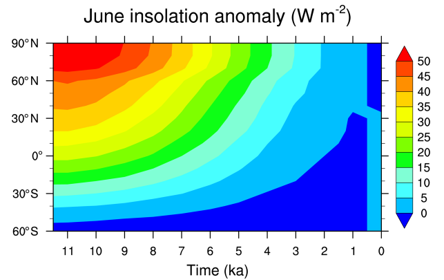
Figure 2. Latitude–time anomalies in the June insolation relative to the average for the last 1000 years, according to Berger (1978).
