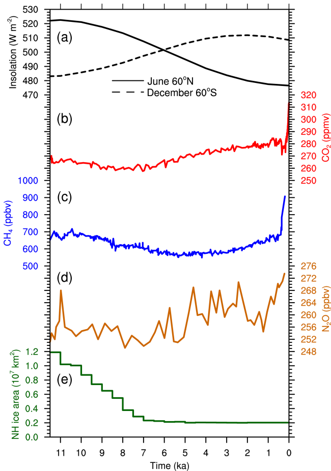
Figure 1. Temporal evolution of the external forcings in the HT-11.5 ka simulations since the Early Holocene (11.5 ka), for (a) June insolation at 60° N (solid line) and December insolation at 60° S (dashed line; Berger, 1978), (b) atmospheric CO 2 concentration (recent composite of EPICA Dome C, Law Dome, and West Antarctic Ice Sheet Divide records, Antarctica; Bereiter et al., 2015), (c) atmospheric CH 4 concentration (EPICA Dome C, Antarctica; Loulergue et al., 2008), (d) Atmospheric N 2 O concentration (Talos Dome, Antarctica; Schilt et al., 2010), and (e) area of the ice sheets in the Northern Hemisphere, according to the ICE-6G_C reconstruction (Argus et al., 2014; Peltier et al., 2015).
