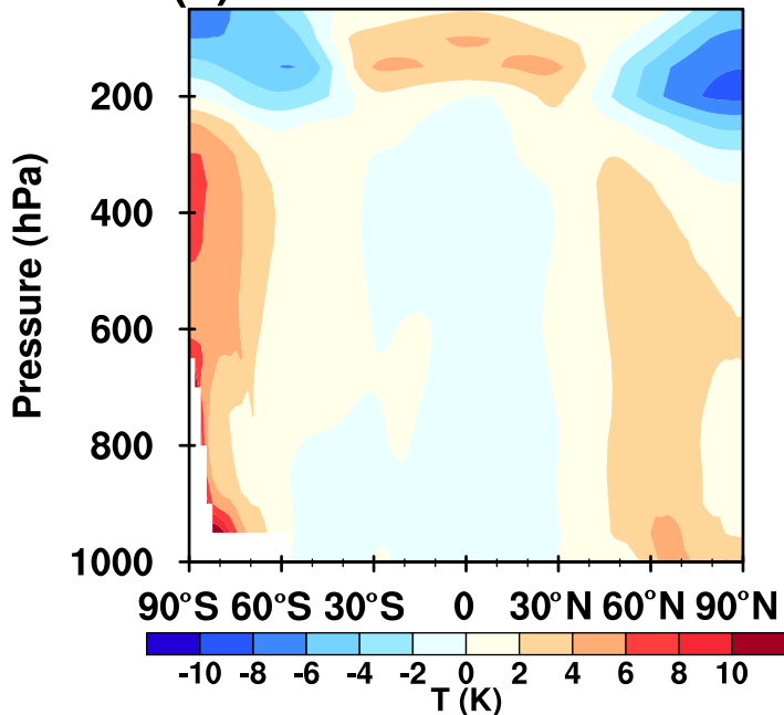
(b) Diff CAM5 Bias:-0.650
