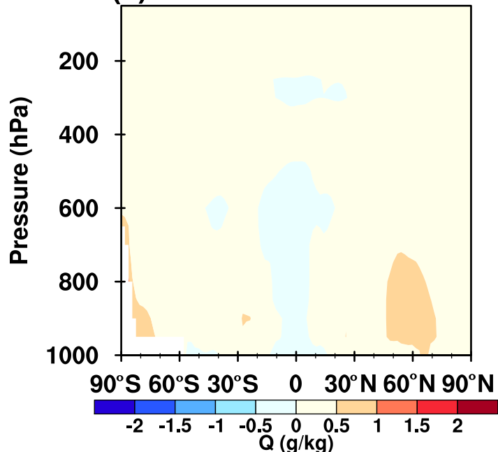
(d) Diff CAM5 Bias:-0.006
