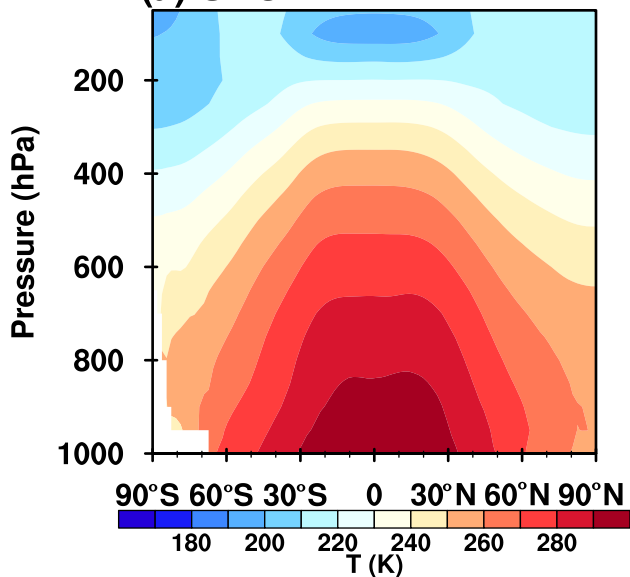
(c) NNCAM RMSE:2.567
