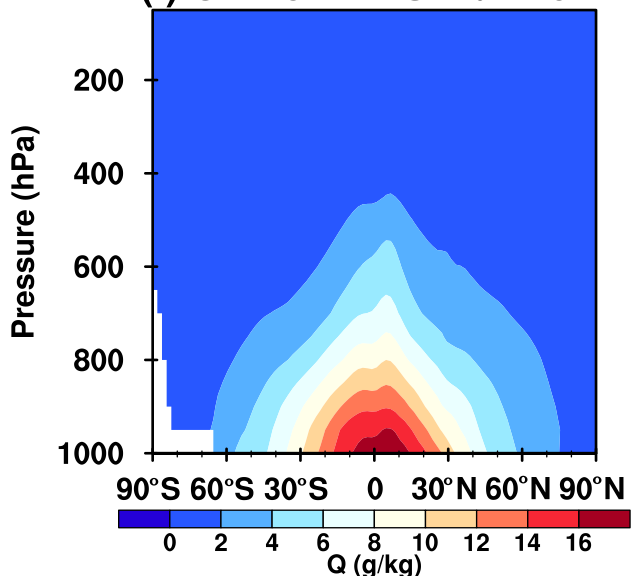
(f) CAM5 RMSE:0.116
