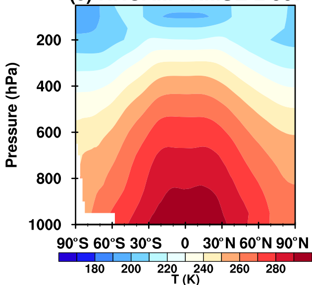
(e) CAM5 RMSE:1.357
