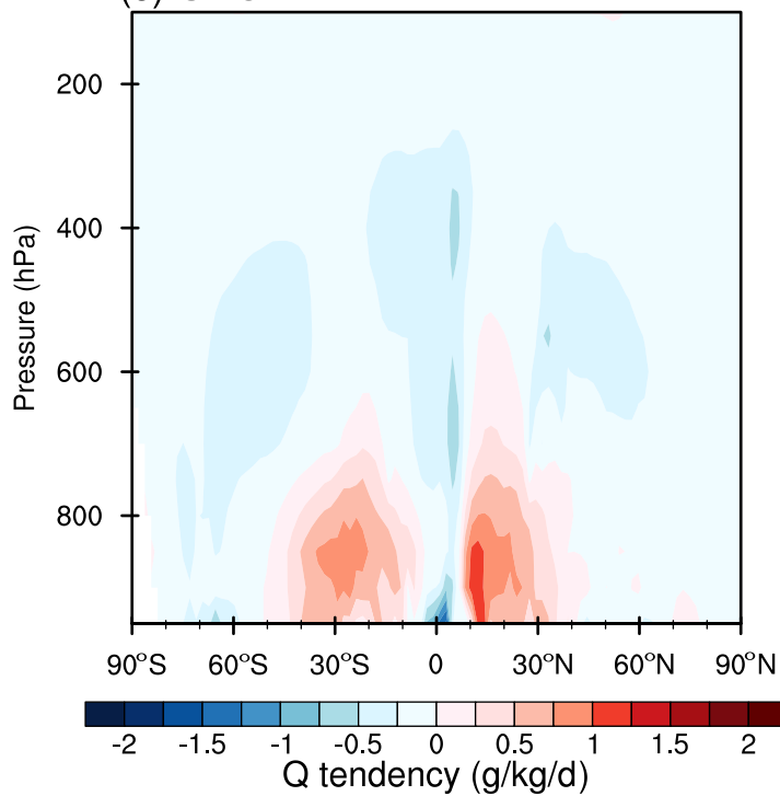
(c) SPCAM
