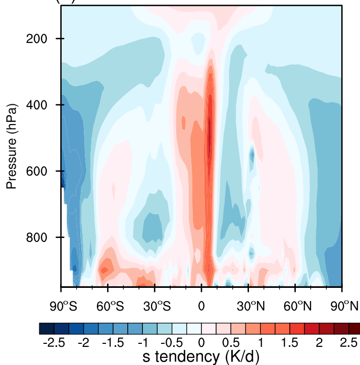
(c) SPCAM
