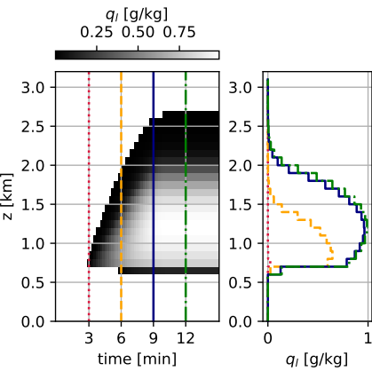
MPDATA iterations: 1
