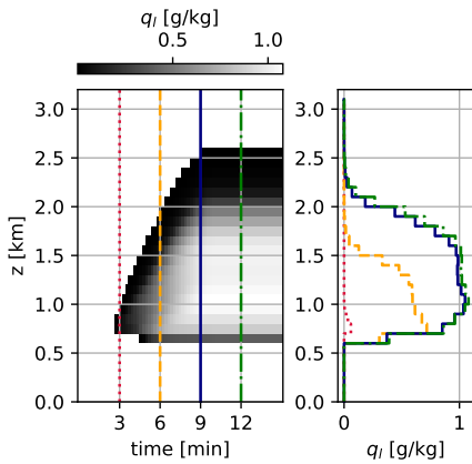
MPDATA iterations: 2
