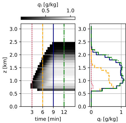
MPDATA iterations: 3
