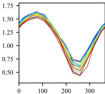
(e) SH CICE extent
