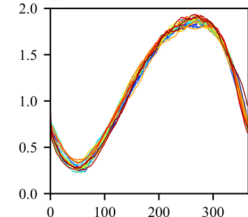
(i) NH PIOMAS volume
