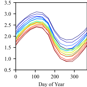
(h) NH CICE volume
