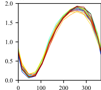
(h) NH CICE volume
