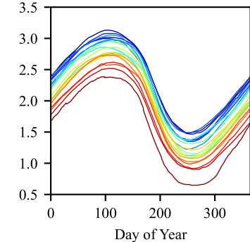
(i) NH PIOMAS volume
