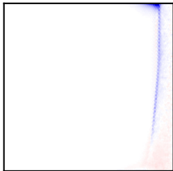
(e) \Delta(\nabla \cdot \sigma)_u PWL
