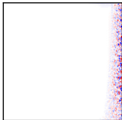
(f) \Delta(\nabla \cdot \sigma)_u FV
