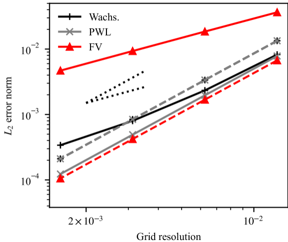
(a) (\nabla \cdot \sigma)_u
