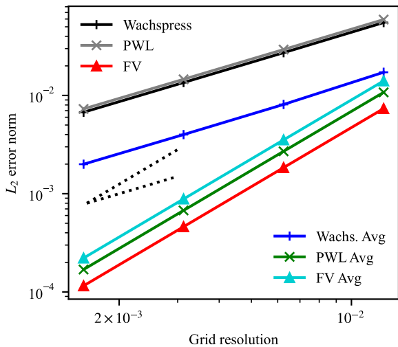
(c) Hex. \partial f/\partial x
