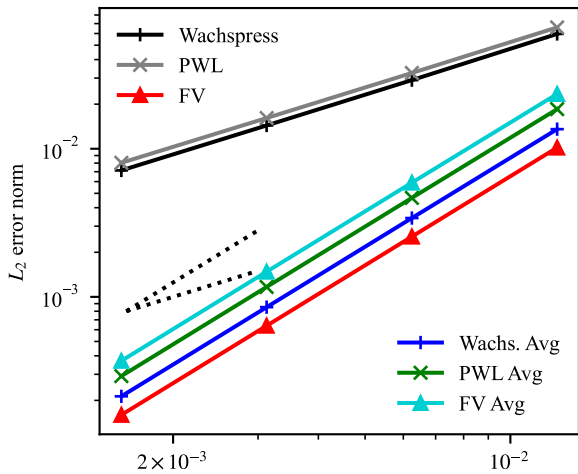
(c) Hex. \partial f/\partial x
