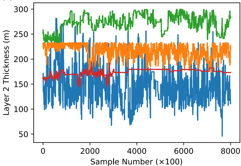
(a) Chain Traces for Model 5 (Aliased)
