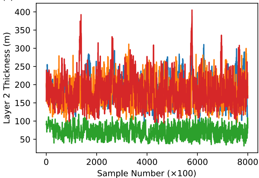
(b) Chain Traces for Model 5 (Anti-Aliased)
