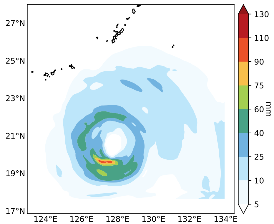
(f) Zhang-McFarlane (cu = 7)
