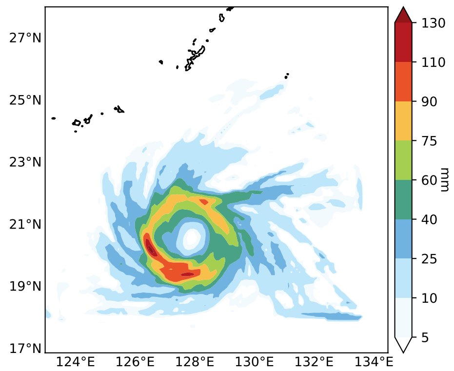
(b) Kain-Fritsch (cu = 1)
