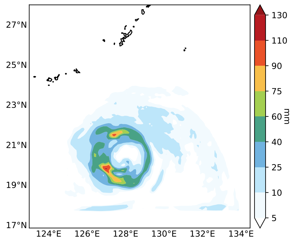
(e) Tiedtke (cu = 6)
