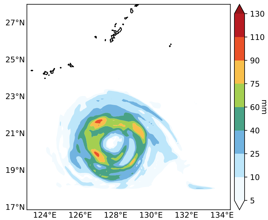
(c) Grell-Freitas (cu = 3)
