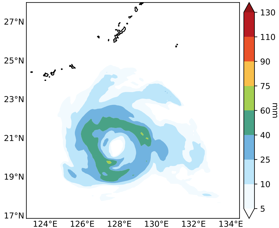
(a) New Tiedtke (cu = 16)
