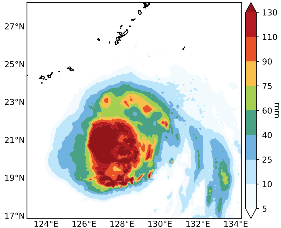
(b) GPM IMERG Final
