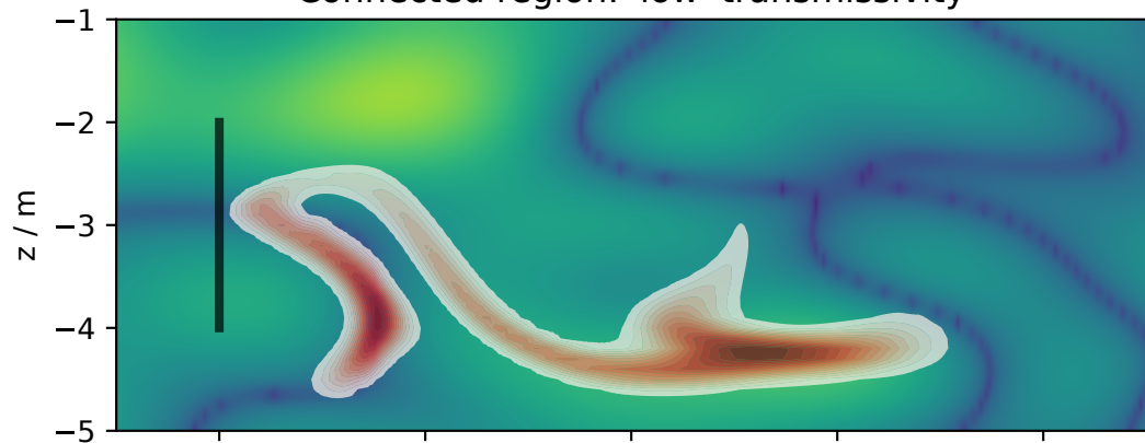
Connected region: 'low' transmissivity
