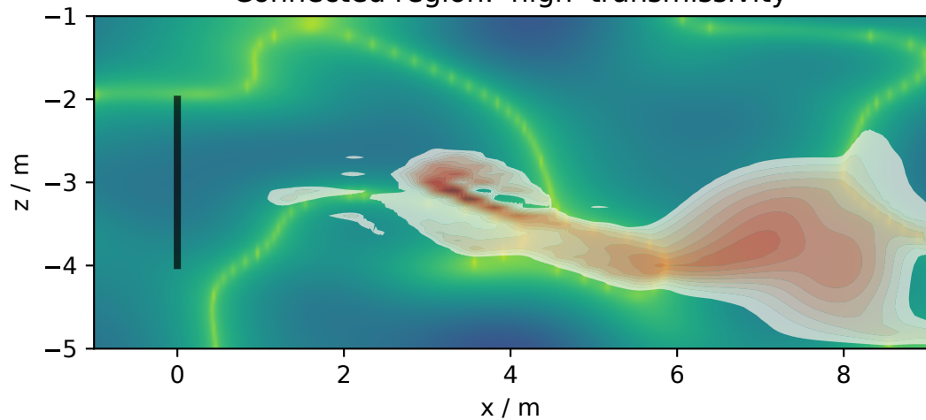
Connected region: 'high' transmissivity
