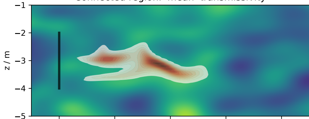
Connected region: 'mean' transmissivity
