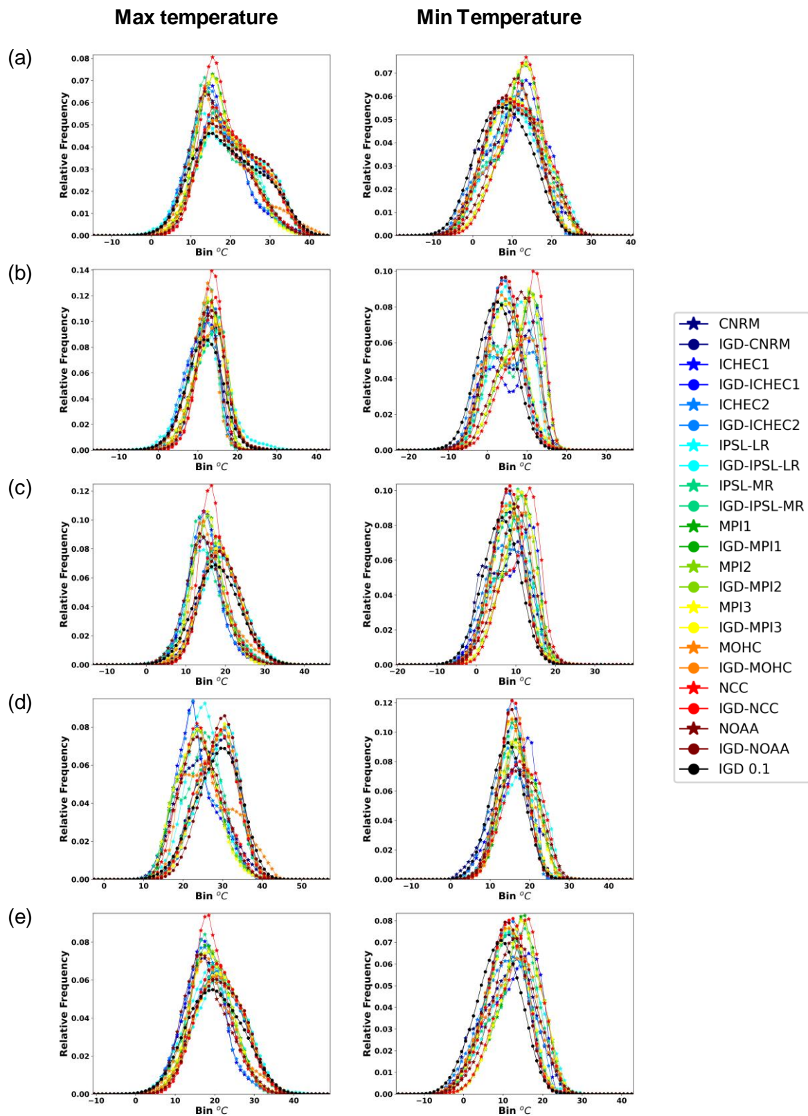
Figure S4. Maximum (left) and minimum (right) daily temperature distributions for the historical driving CMIP5 GCMs and IGD observations interpolated into each GCM resolution for the Iberian Peninsula, considering the 1971-2005 period. Also shown the PDF from the IGD observations at the original resolution. (a) Year, (b) DJF, (c) MAM, (d) JJA and (e) SON.
