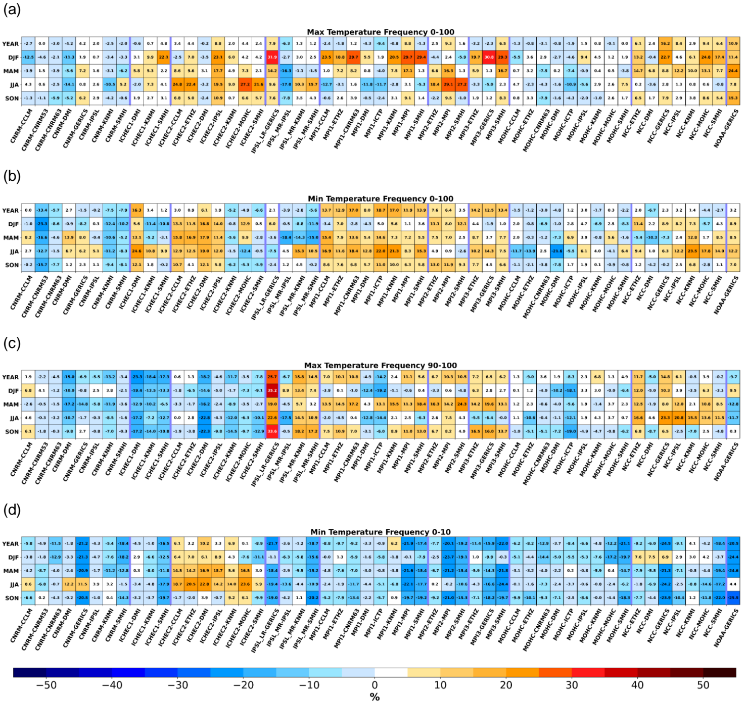
Figure S5. Yearly and seasonal distribution added values (DAV) of the Iberian Peninsula, between the RCMs and the CMP5 GCMs for the 1989-2008 period, taken from the Historical EURO-CORDEX simulations, with the IGD regular dataset as a reference for (a) maximum daily temperature, considering the whole PDF shown in the left panels of Figure S3, (b) minimum daily temperature considering the whole PDF shown in the right panels of Figure S3, (c) maximum daily temperature extremes, only considering the values above the observational 90 th percentile from maximum temperatures and (d) minimum daily temperature extremes, only considering the values below the observational 10 th percentile from minimum temperatures. All model data were previously interpolated to 0.1° regular resolution from the observations. The thick blue lines separate the RCMs driven by different GCM.
