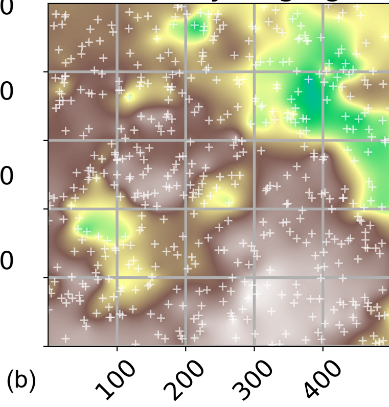
Ordinary Kriging
