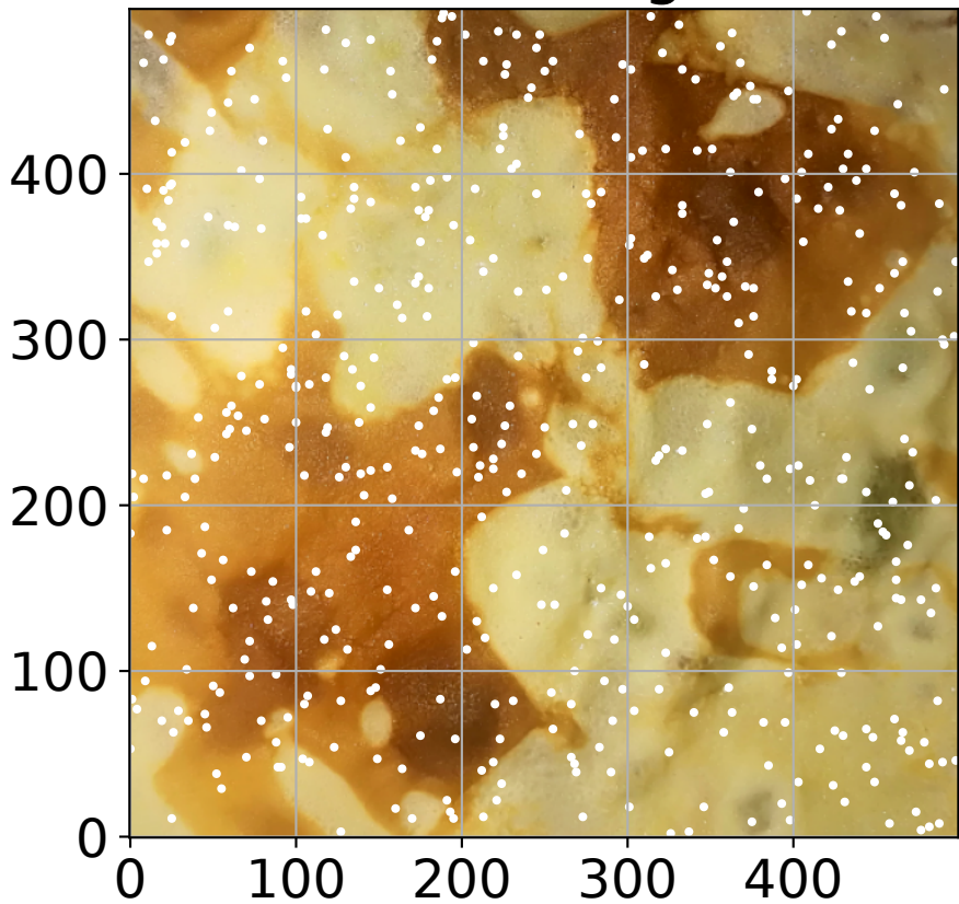
RGB image
