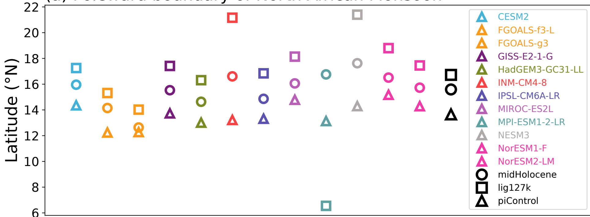
(b) Northward monsoon extension
