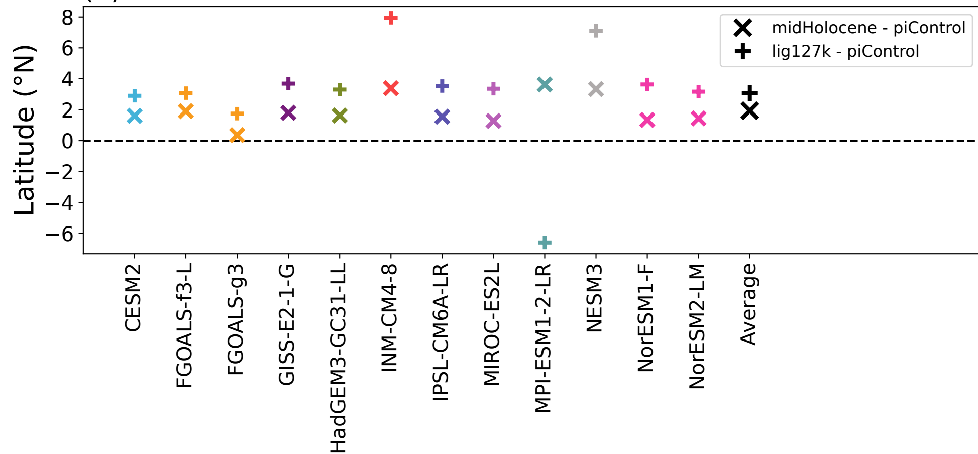
(b) Northward monsoon extension
