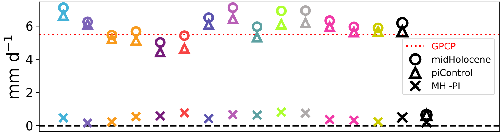
(a) Rainfall over NAF domain
