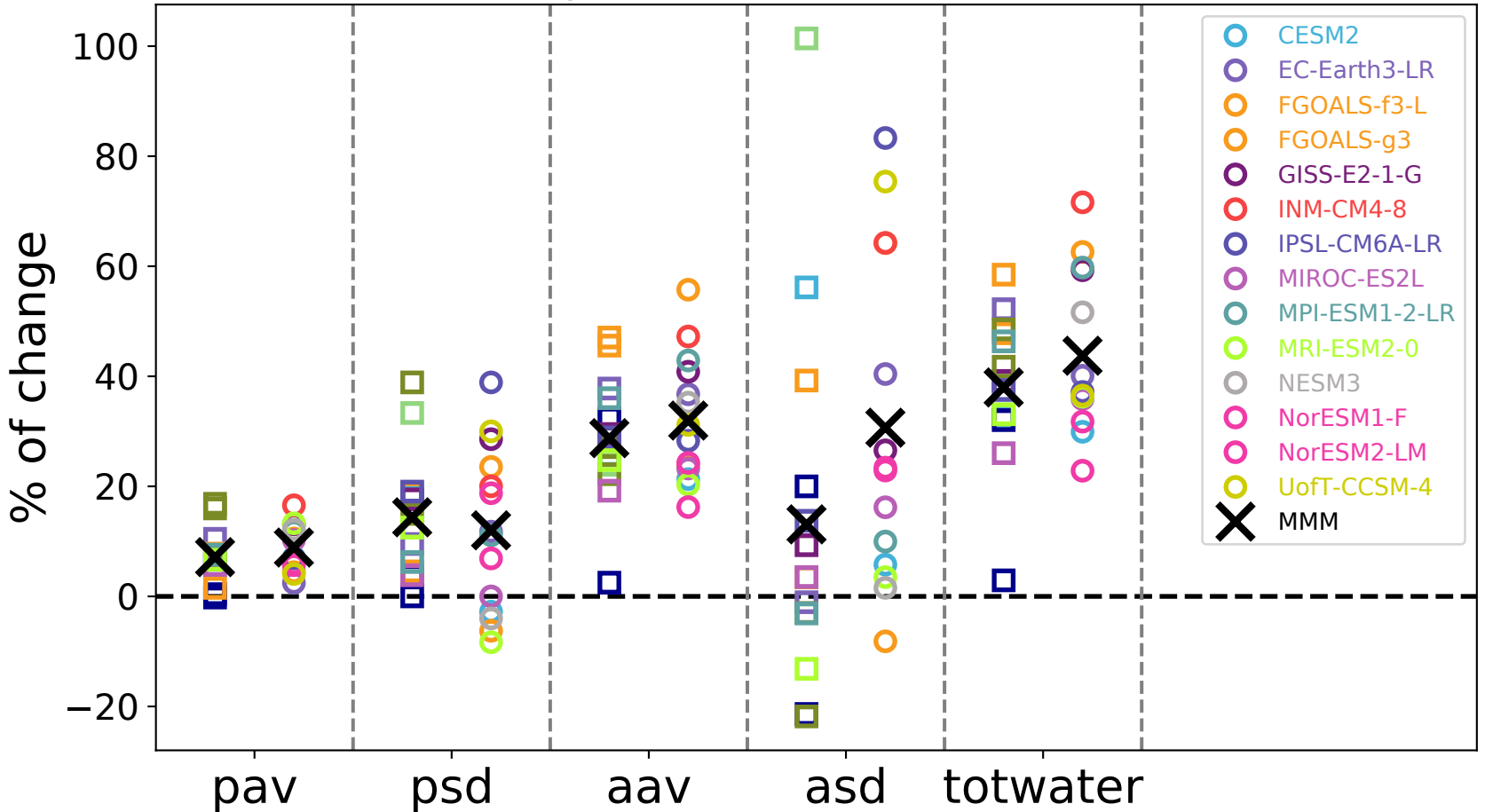
(c) Relative changes in NAF
