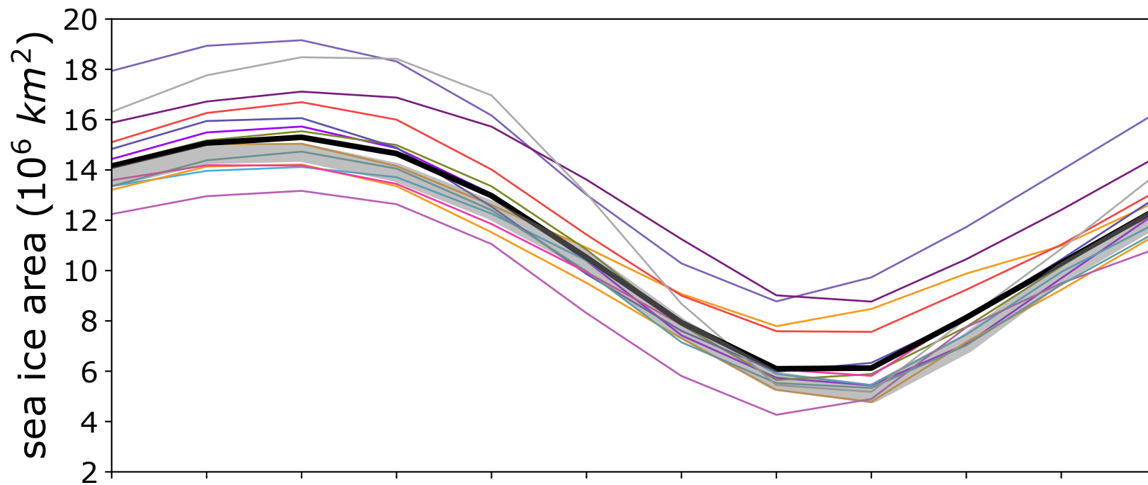
(b) midHolocene NH sea ice area
