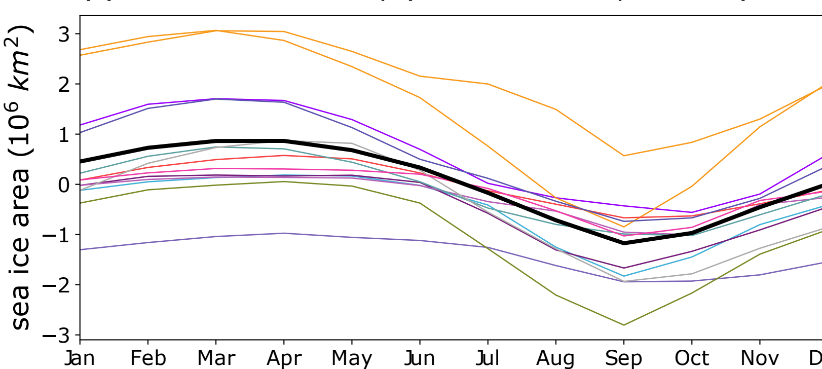
(c) NH sea ice anomaly (midHolocene - piControl)
