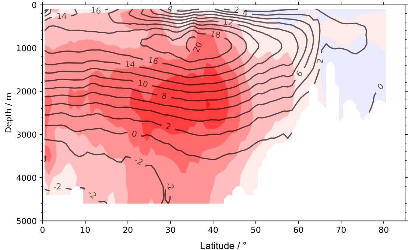
mean (annual) AMOC changes (MH - PI) ensemble mean -- 10 PMIP4 models
