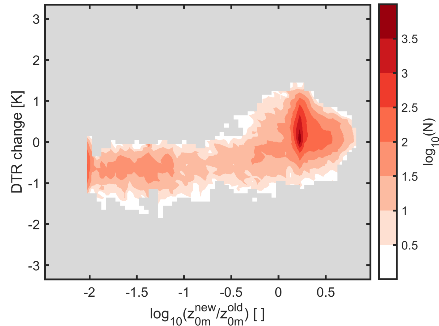
(c) TBOT at grid cell level
