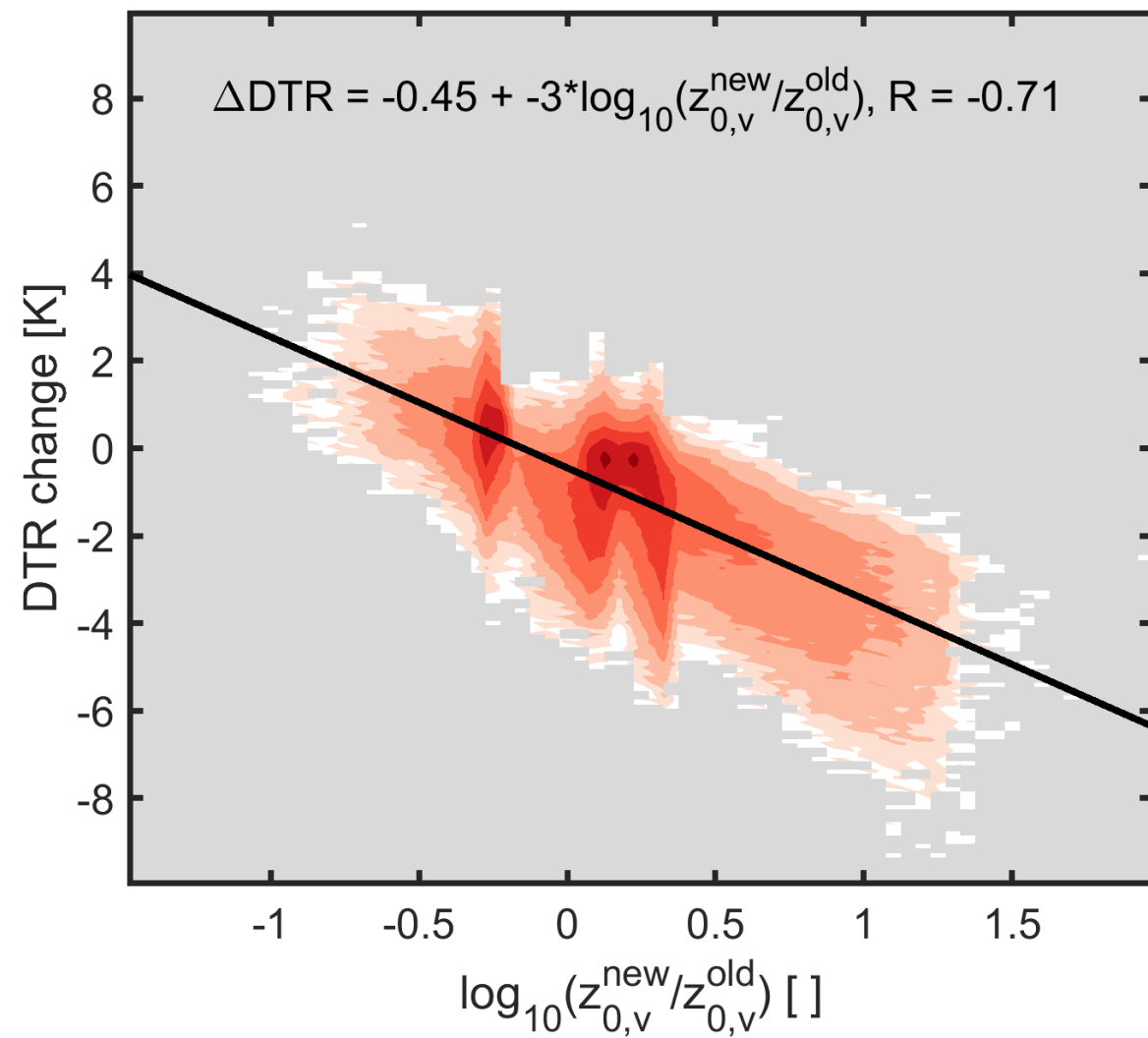
(a) LST at PFT level
