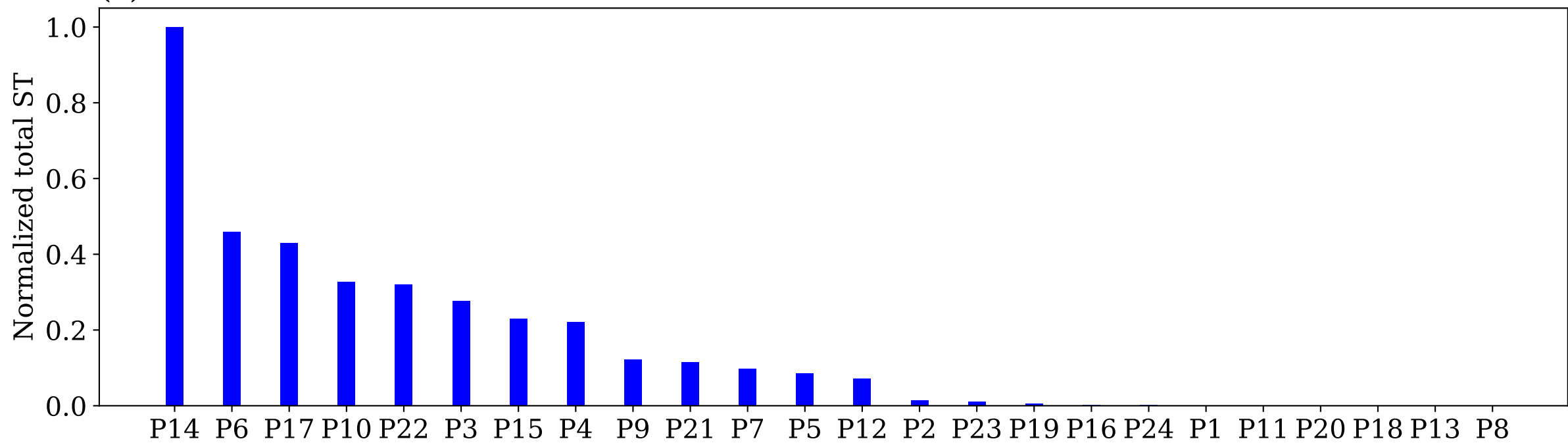
(c) Sobol
