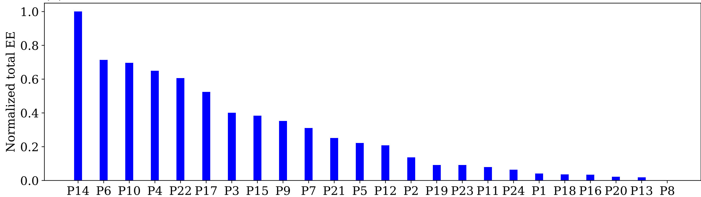
(a) MOAT
