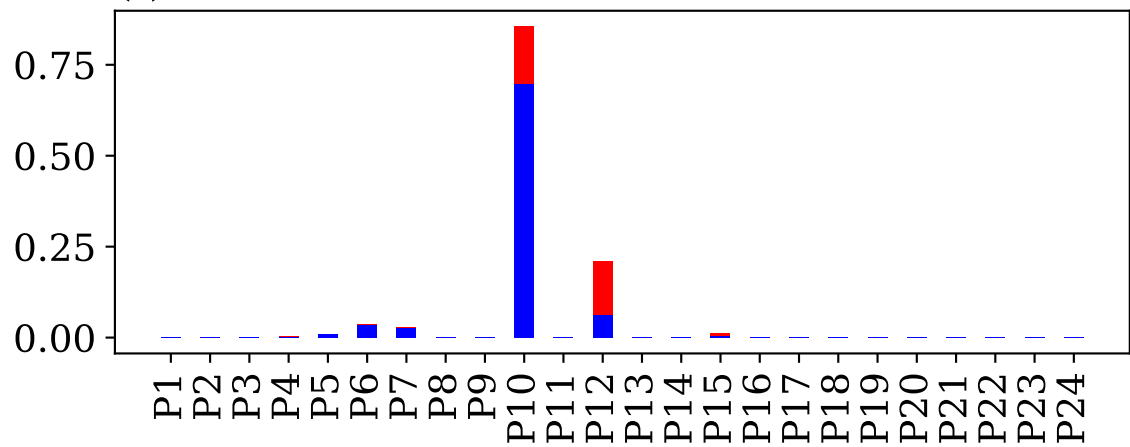
(h) DLWRF
