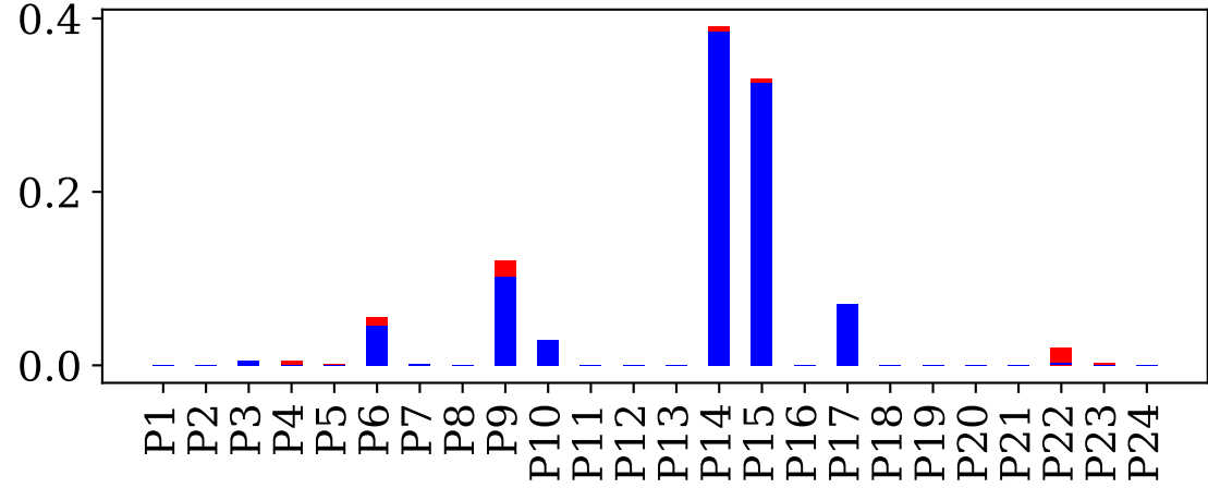
(h) DLWRF
