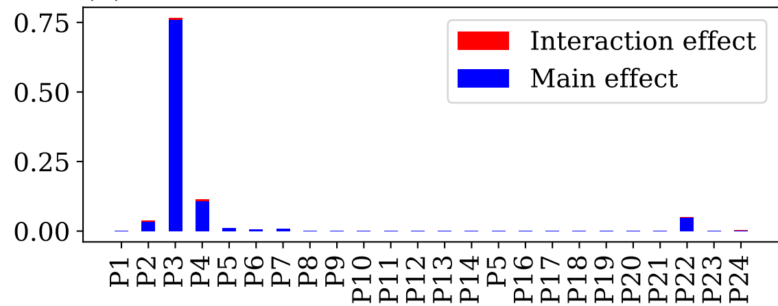
(c) SAP
