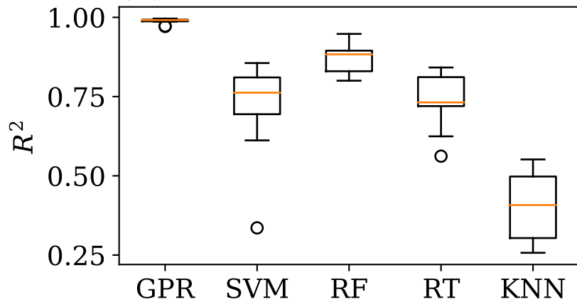
(b) SAT
