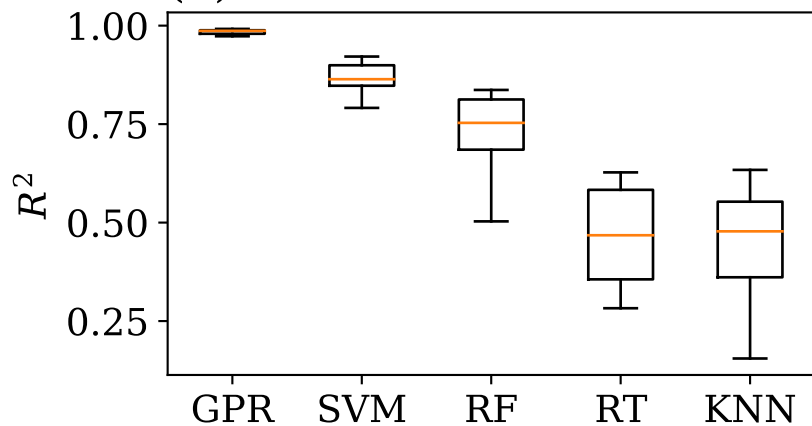
(h) DLWRF
