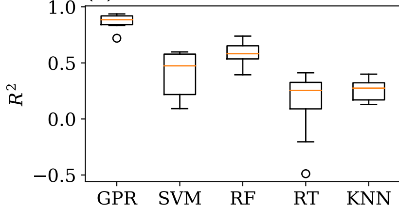
(c) SAP
