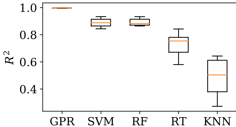
(a) WS10
