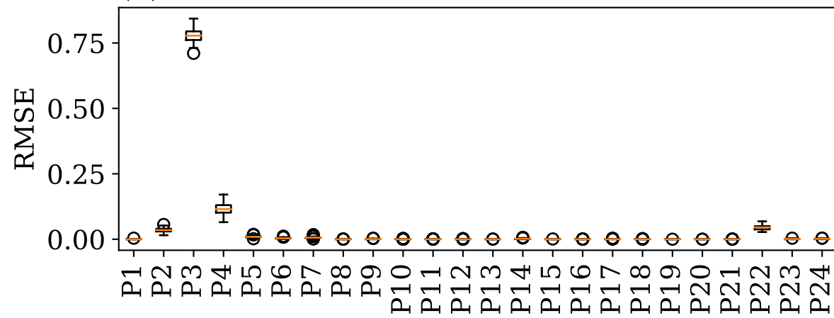
(c) SAP
