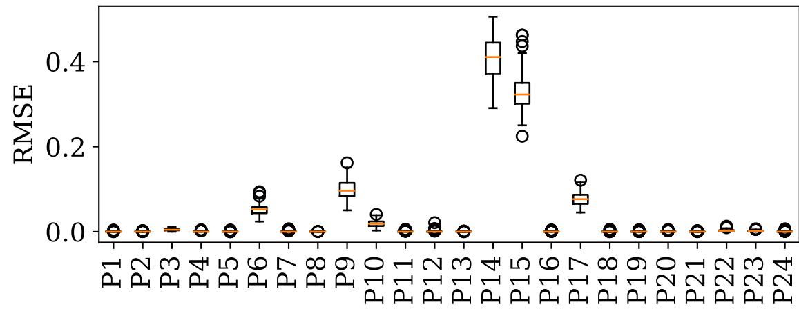
(h) DLWRF
