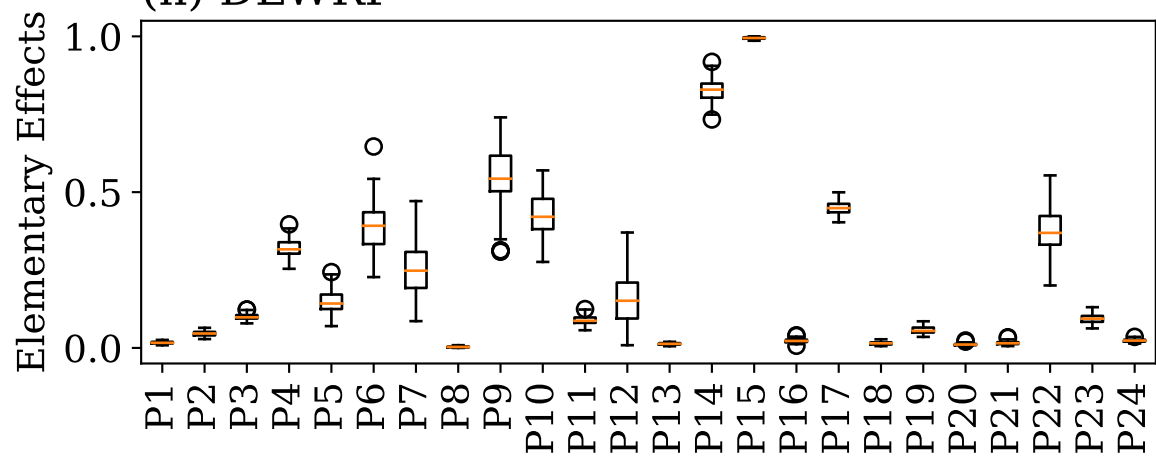
(h) DLWRF
