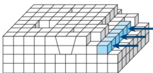
Step-edge retreat
