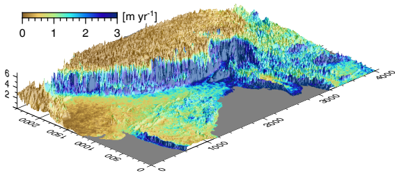
(c) Precipitation TRMM2b31
