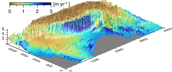
(c) Precipitation TRMM2b31
