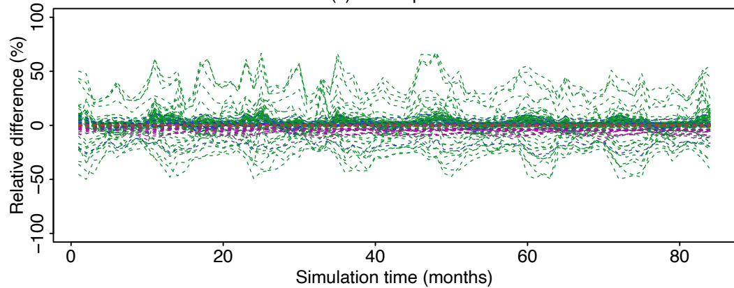
(c) Stratosphere
