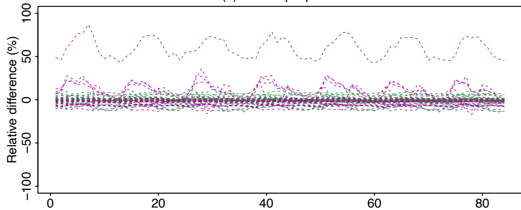
(c) Stratosphere
