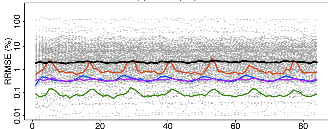
(c) Stratosphere
