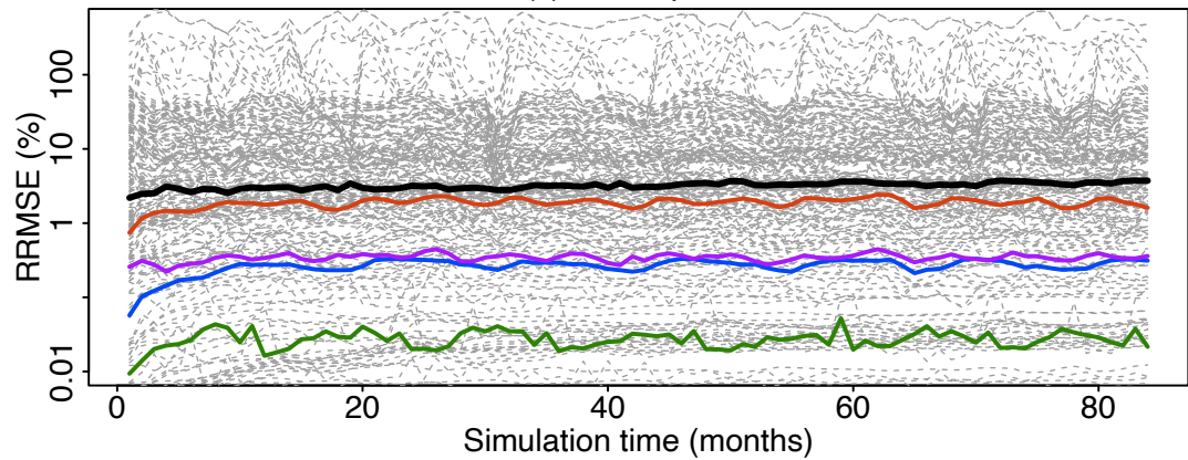
(c) Stratosphere
