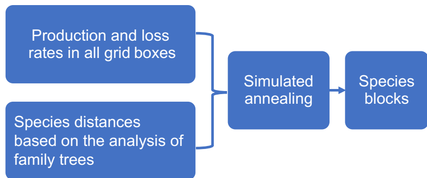
(c) Network of atmospheric species
