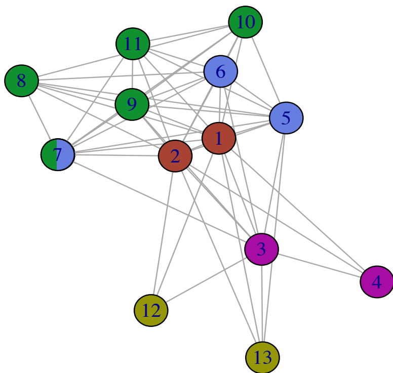
(c) Network of atmospheric species
