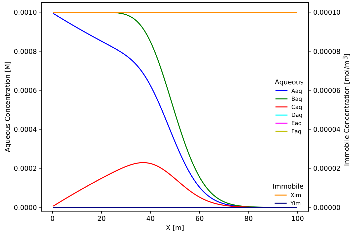
Concentration Profile at 12.5 years
