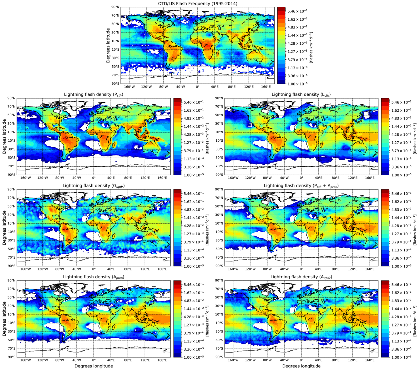
Figure 4. Global annual lightning observations (upper panel) by OTD/LIS using the OTD/LIS Gridded Lightning Climatology Data Collection version 2.3.2015 High-Resolution Monthly Climatology (HRMC) from 4 May 1995 to 31 December 2014 (Christian et al., 2003; Cecil et al., 2014). As in Gordillo-Vázquez et al. (2019), the climatology has been degraded to 2.5^\circ longitude \times 1.9^\circ latitude resolution. Simulated annual average flash density (remaining panels) between 1 March 2017 and 28 February 2018 using different lightning parameterizations described in Table 1.
