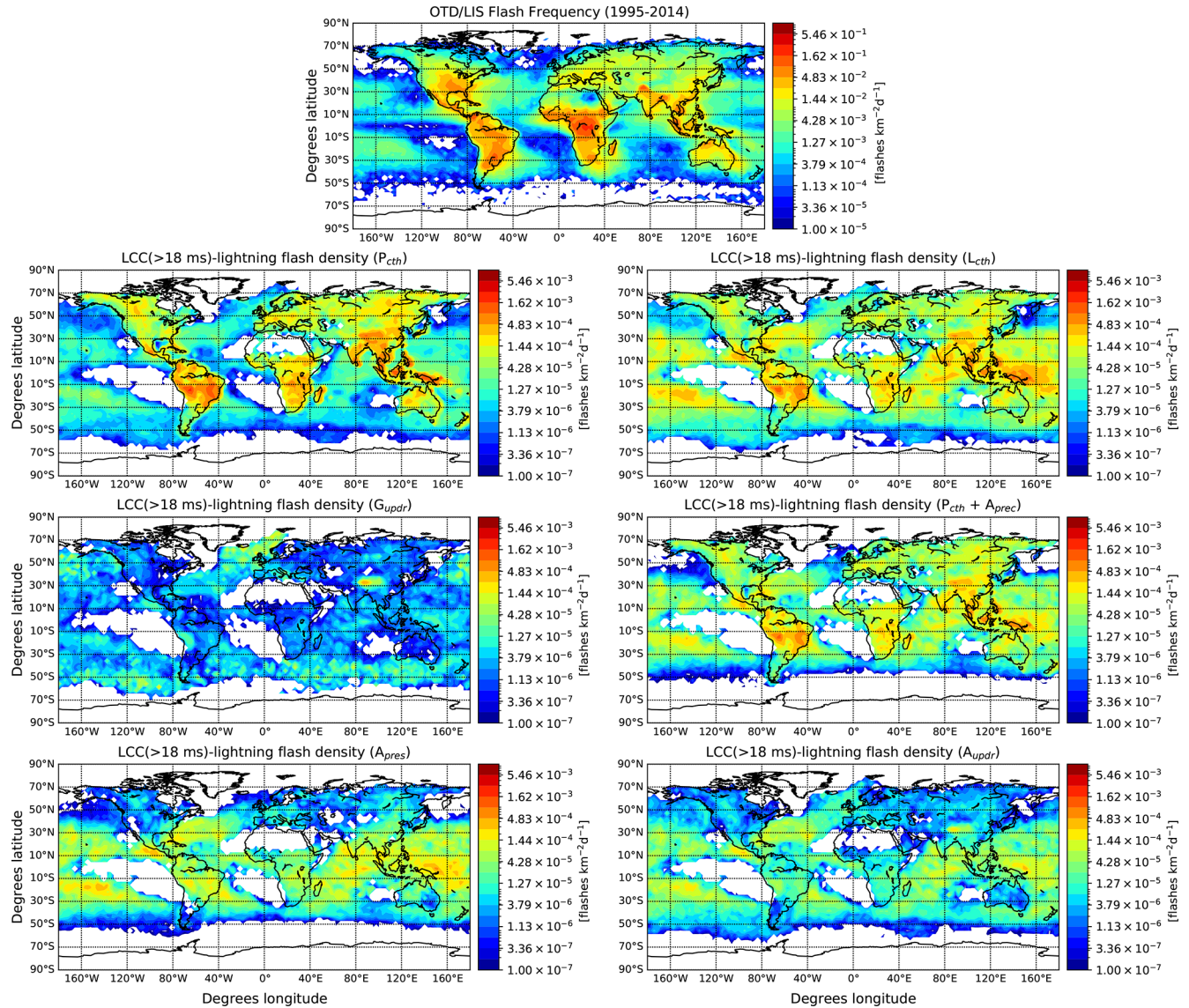
Figure 6. Global annual lightning observations (upper panel) by OTD/LIS as in Fig. 4. Simulated annual average LCC(> 18 ms) lightning flash density (remaining panels) between 1 March 2017 and 28 February 2018 using different lightning parameterizations.
