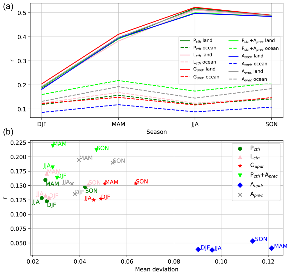
Figure 13. Seasonal evolution of the spatial correlation coefficient ( r ) between the observed and simulated ratio of LCC(> 9 ms) lightning to total lightning for land and ocean (a) as well as the seasonal global correlation coefficient versus the deviation averaged over all the grid cells between the observed and simulated ratio of LCC(> 9 ms) lightning to total lightning (b). Each point represents a different season.
