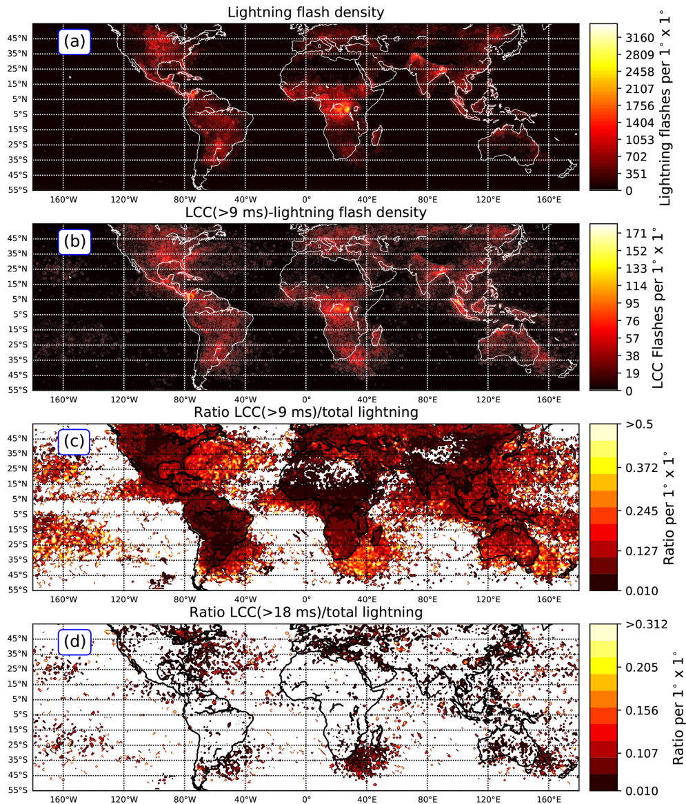
Figure 1. Annual lightning flash density (a), LCC(> 9 ms) lightning flash density (b), ratio between LCC(> 9 ms) lightning and lightning flash densities (c), and ratio between LCC(> 18 ms) lightning and lightning flash densities (d) extracted from ISS LIS data between March 2017 and March 2018 binned into 1^\circ \times 1^\circ grids. The ratio is undefined in grids without any detection of LCC lightning flashes.
