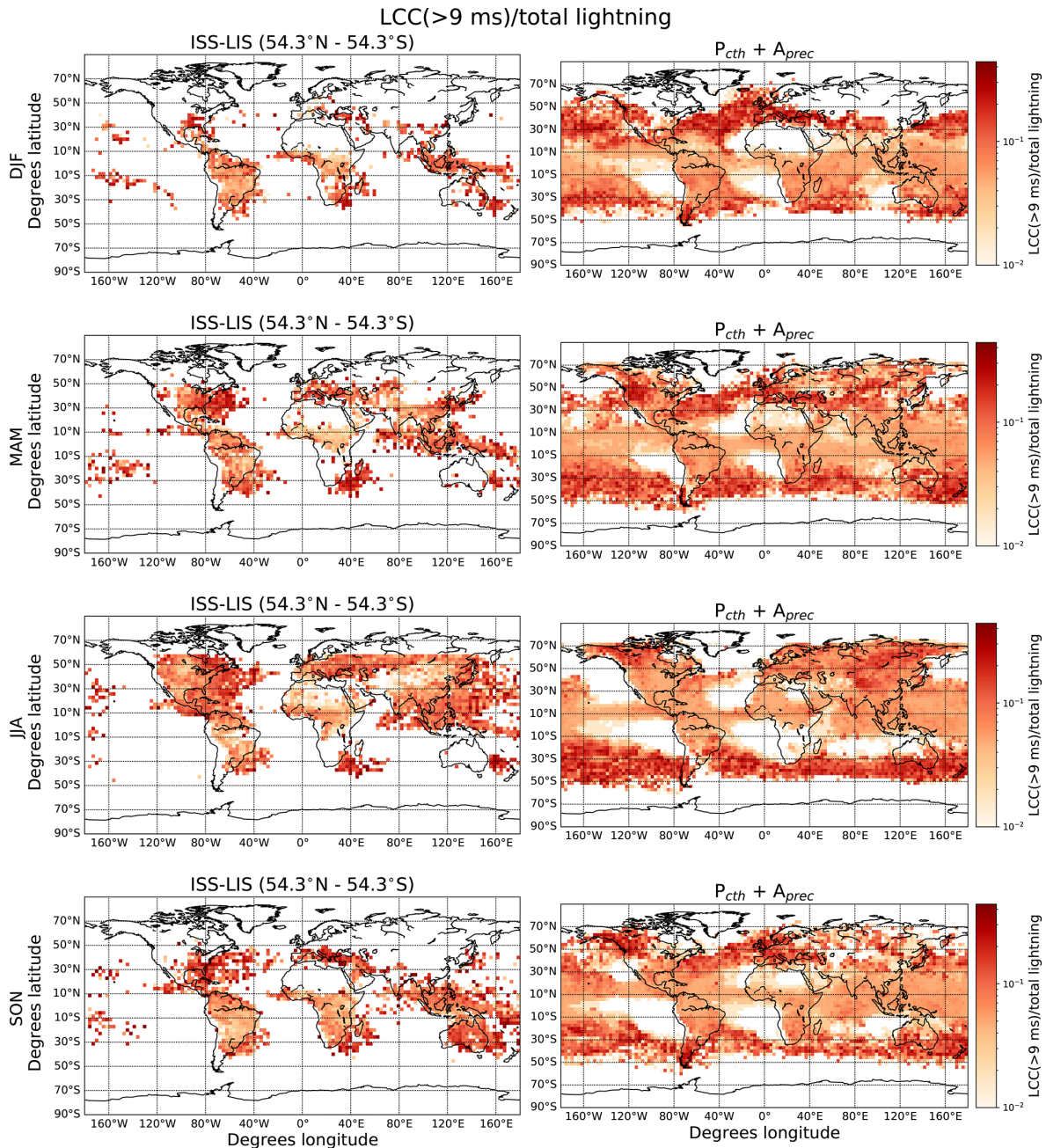
Figure 7. Seasonal observed (left panels) and simulated (right panels) ratio of LCC(> 9 ms) lightning to total lightning using the P_{cth} + A_{prec} lightning parameterization. The maximum value of the color bar is 0.44.
