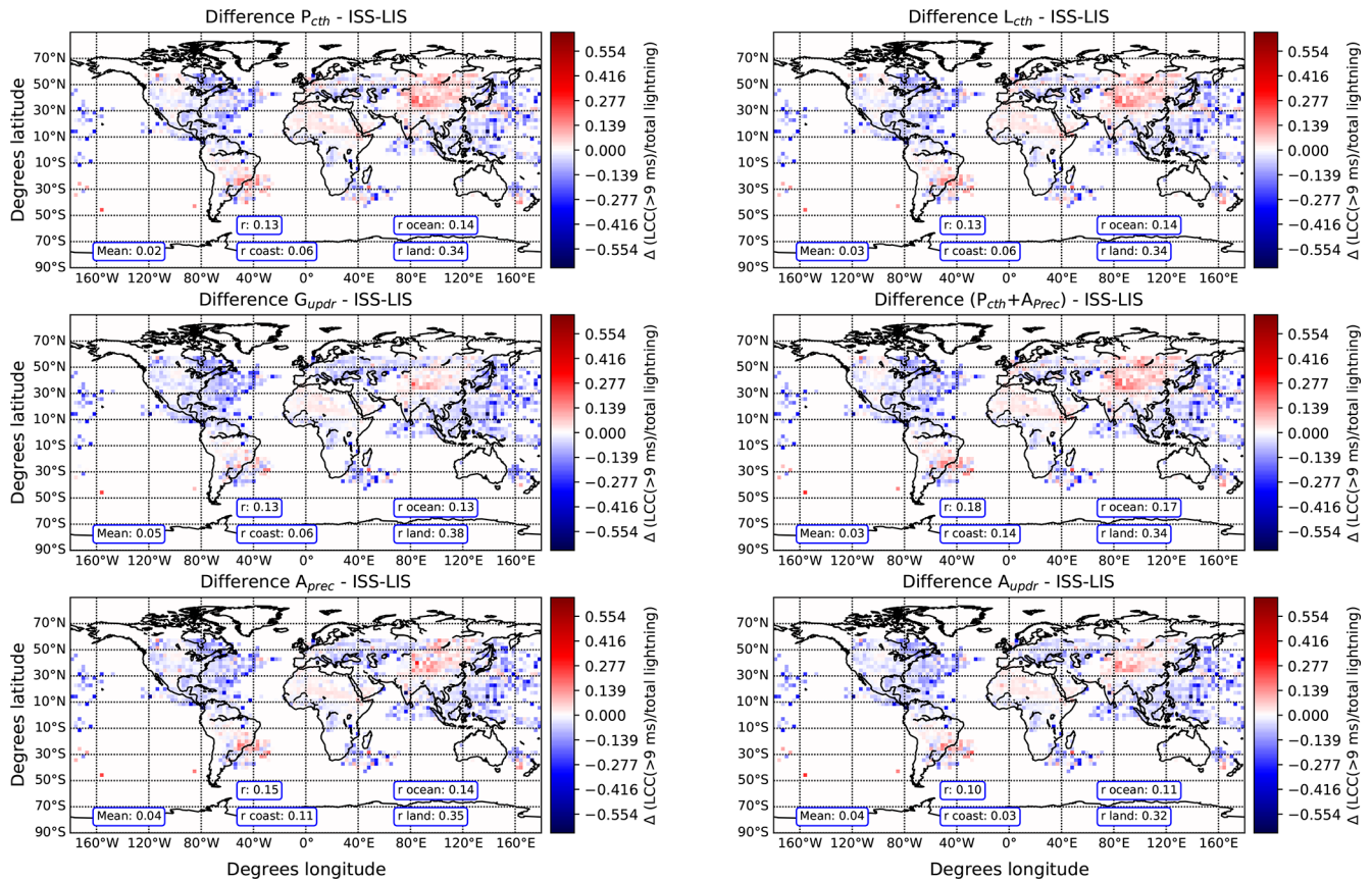
Figure 11. Difference between the observed and simulated ratio of LCC(> 9 ms) lightning to total lightning density in June, July, and August using different lightning parameterizations. Positive values indicate that the model overestimates the ratio. The calculated global, land, and ocean spatial correlation coefficients r are included.
