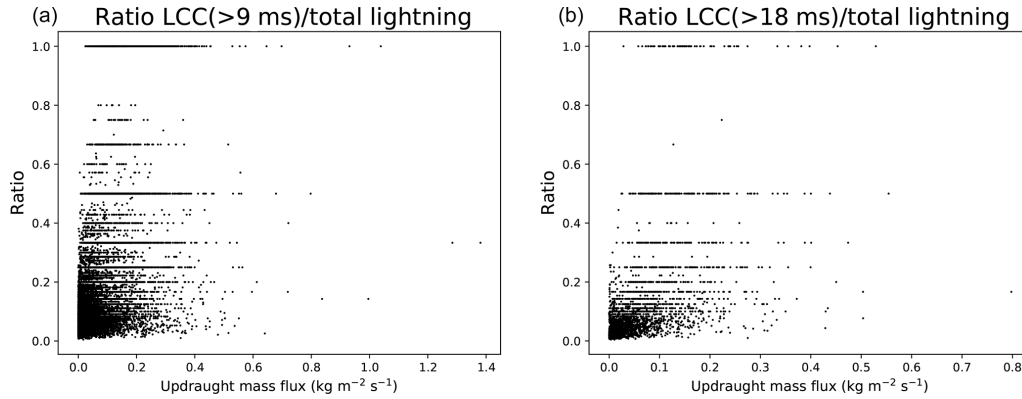
Figure 2. Ratios of (a) LCC(> 9 ms) and (b) LCC(> 18 ms) lightning to total lightning flashes versus the updraft mass flux extracted from ERA5 1-hourly averaged 2.75^\circ \times 2.75^\circ grid cells for lightning reported by ISS LIS globally between March 2017 and March 2018.
