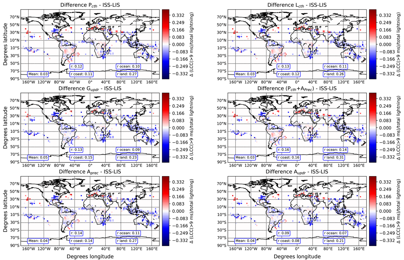
Figure 9. Difference between the observed and simulated ratio of LCC(> 9 ms) lightning to total lightning density in December, January, and February using different lightning parameterizations. Positive values indicate that the model overestimates the ratio. The calculated global, land, and ocean spatial correlation coefficients r are included.
