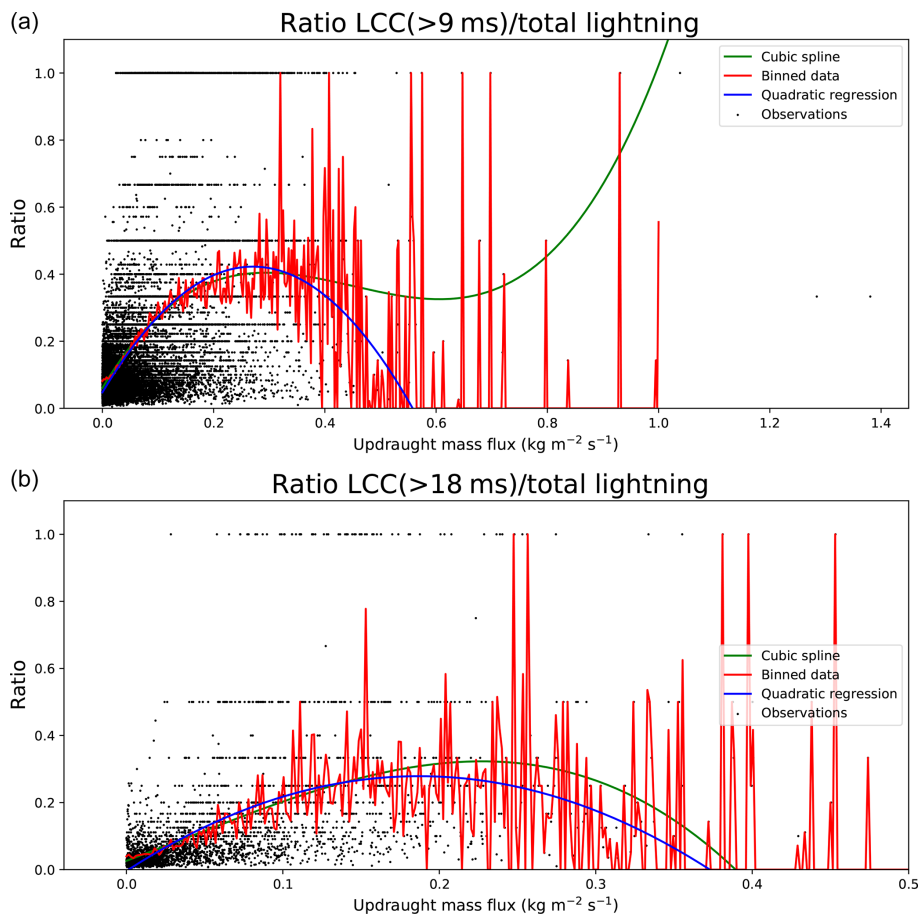
Figure 3. Ratios of (a) LCC(> 9 ms) and (b) LCC(> 18 ms) lightning to total lightning flashes versus the updraft mass flux as in Fig. 2. We have added a cubic smoothing spline (green line), a quadratic fitting (blue line), and a binning (red line) to the data as described in the text.
