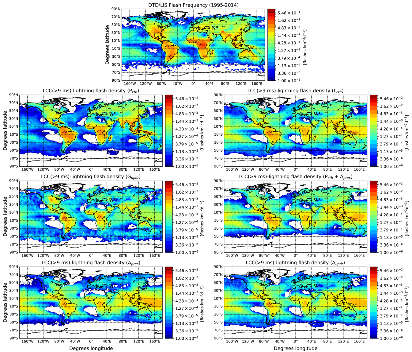
Figure 5. Global annual lightning observations (upper panel) by OTD/LIS as in Fig. 4. Simulated annual average LCC(> 9 ms) lightning flash density (remaining panels) between 1 March 2017 and 28 February 2018 using different lightning parameterizations.
