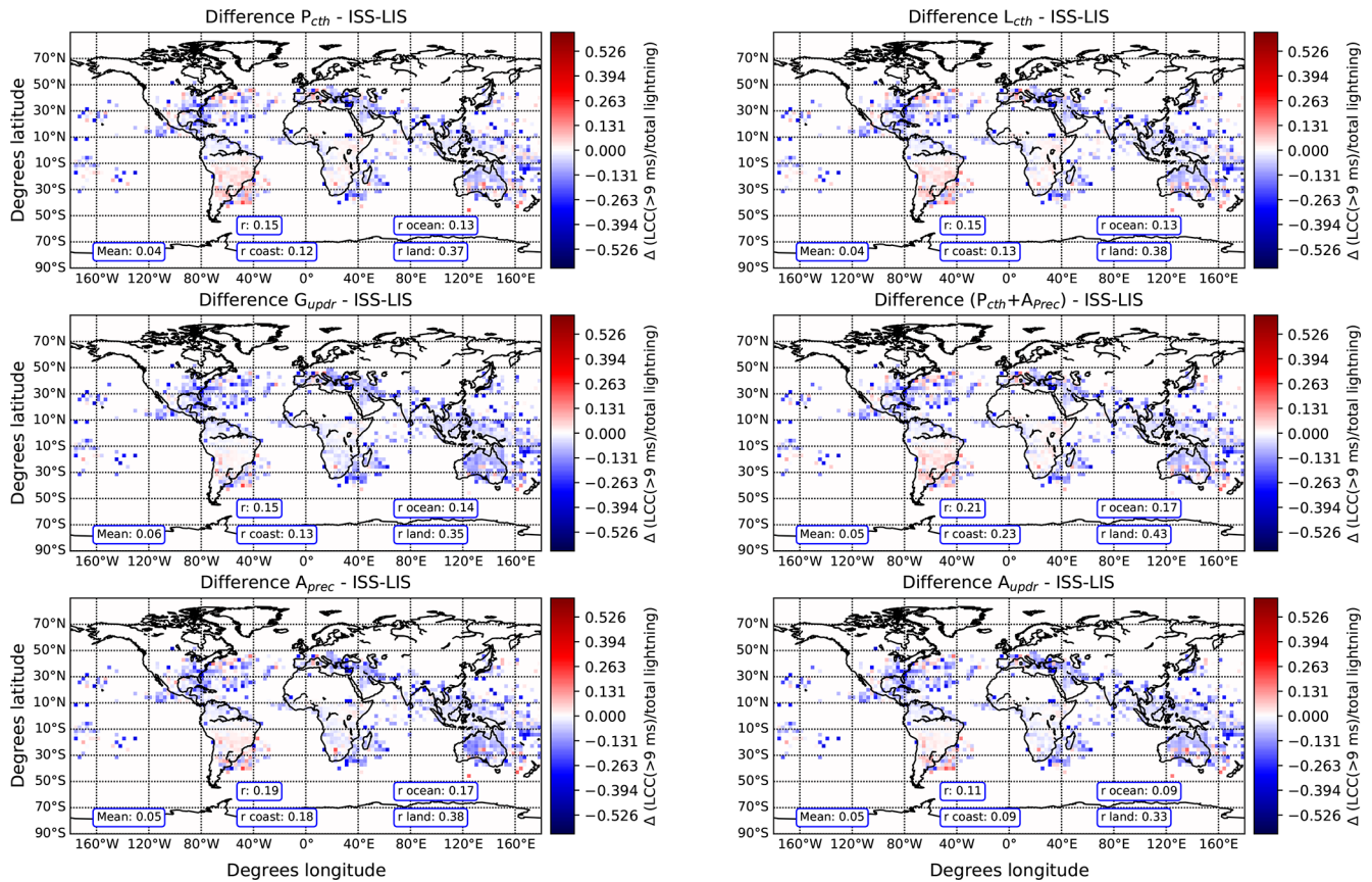
Figure 12. Difference between the observed and simulated ratio of LCC(> 9 ms) lightning to total lightning density in September, October, and November using different lightning parameterizations. Positive values indicate that the model overestimates the ratio. The calculated global, land, and ocean spatial correlation coefficients r are included.
