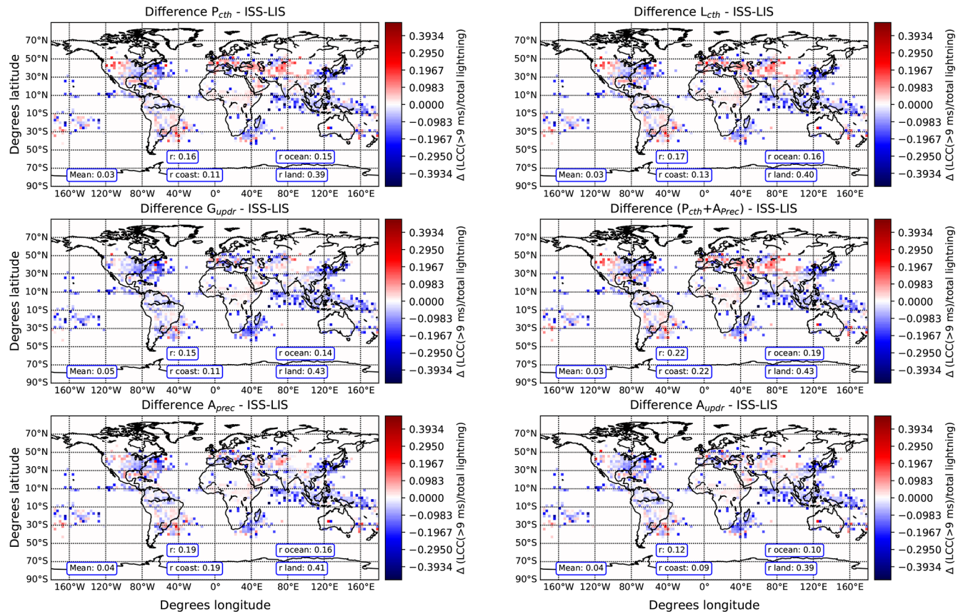
Figure 10. Difference between the observed and simulated ratio of LCC(> 9 ms) lightning to total lightning density in March, April, and May using different lightning parameterizations. Positive values indicate that the model overestimates the ratio. The calculated global, land, and ocean spatial correlation coefficients r are included.
