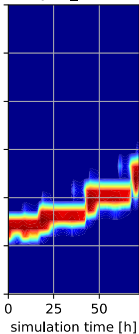
cy40_NEW
