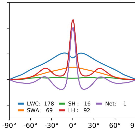
(e) GA7.0 slab ocean: budget
