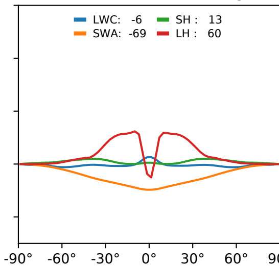
(f) Flex-UM - GA7.0: budget
