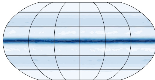
(b) GA7.0 slab ocean: P
