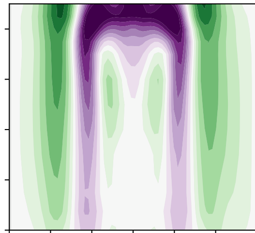
(f) Flex-UM - GA7.0: \Psi
