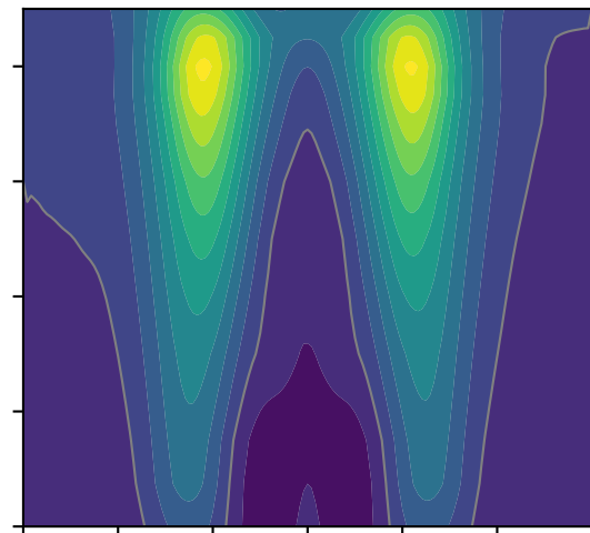
(e) GA7.0 slab ocean: \Psi
