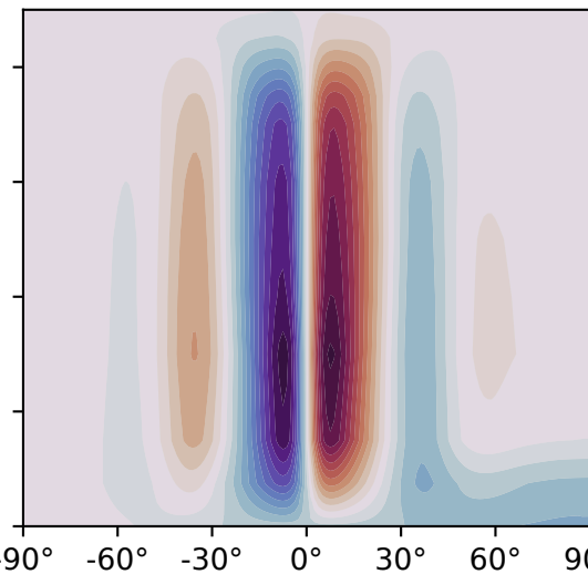
(e) GA7.0 slab ocean: \Psi
