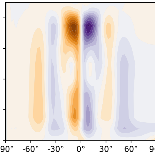
(f) Flex-UM - GA7.0: \Psi
