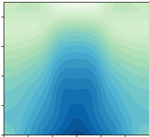
(e) GA7.0 slab ocean: RH
