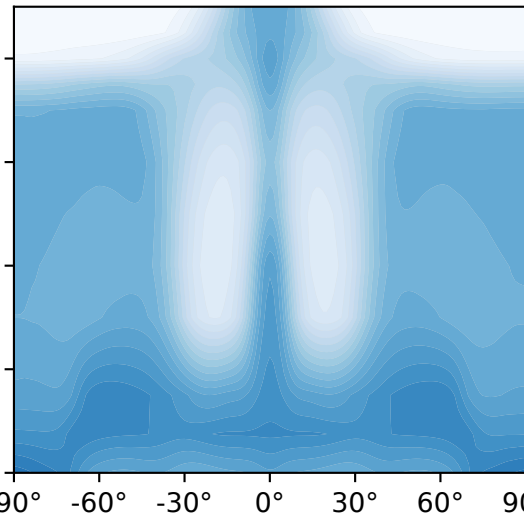
(e) GA7.0 slab ocean: RH
