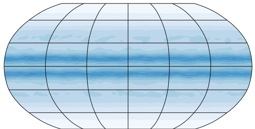
(a) Flex-UM fixed SST: P
