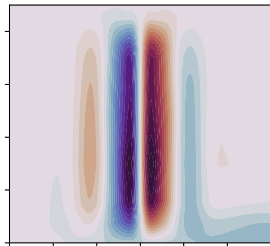
(e) GA7.0 fixed SST: \Psi
