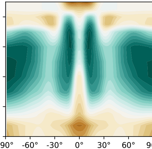
(f) Flex-UM - GA7.0: RH
