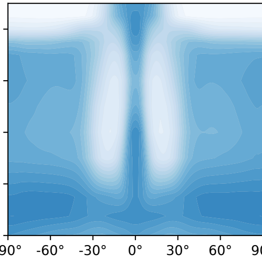
(e) GA7.0 fixed SST: RH
