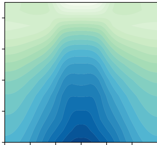
(e) GA7.0 fixed SST: RH
