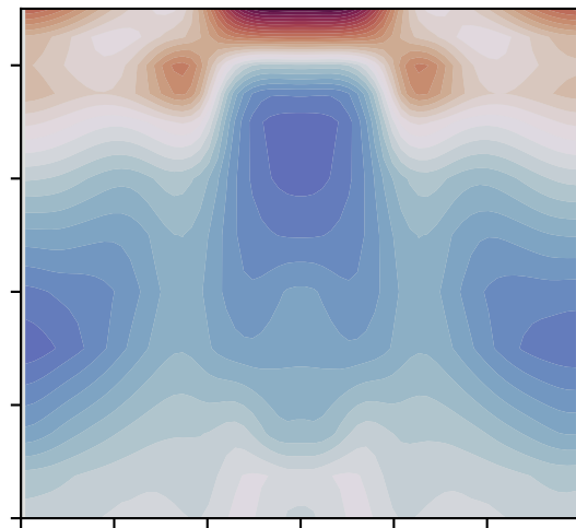
(f) Flex-UM - GA7.0: RH
