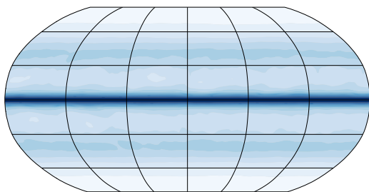
(b) Isca slab ocean: P
