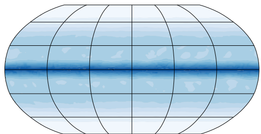
(a) Flex-UM slab ocean: P
