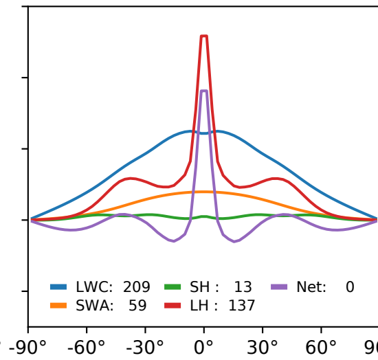
(e) Isca slab ocean: budget
