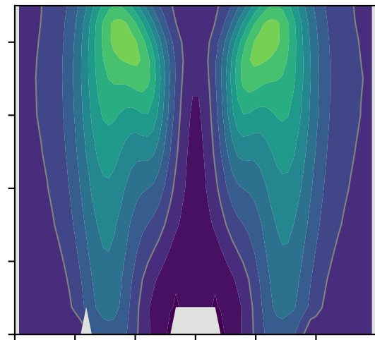
(e) Isca slab ocean: \Psi
