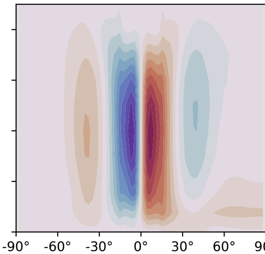
(e) Isca slab ocean: \Psi
