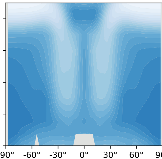
(e) Isca slab ocean: RH
