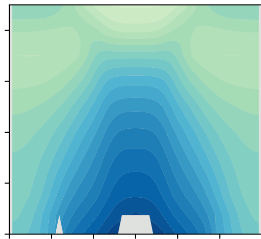
(e) Isca slab ocean: RH
