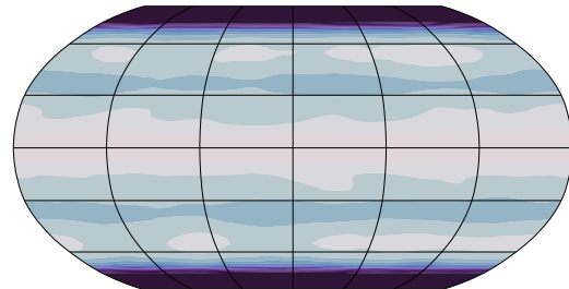
(f) GA7.0 Slab - Fixed SST: SST
