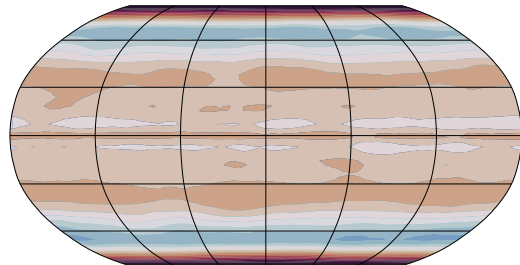
(e) Flex-UM Slab - GA7.0 Slab
