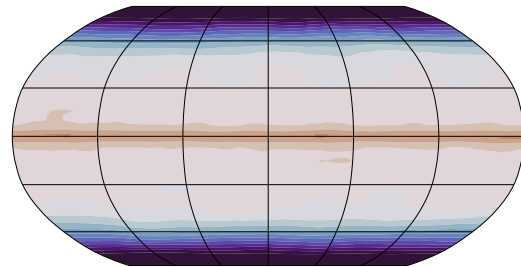
(c) Flex-UM Slab - Fixed SST: SST
