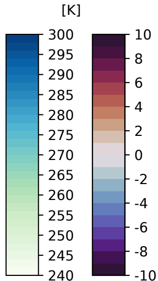
(f) GA7.0 Slab - Fixed SST: SST
