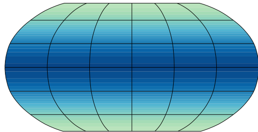
(b) fixed SST: SST
