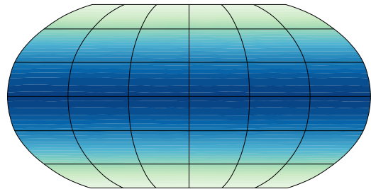
(a) Flex-UM Slab ocean: SST
