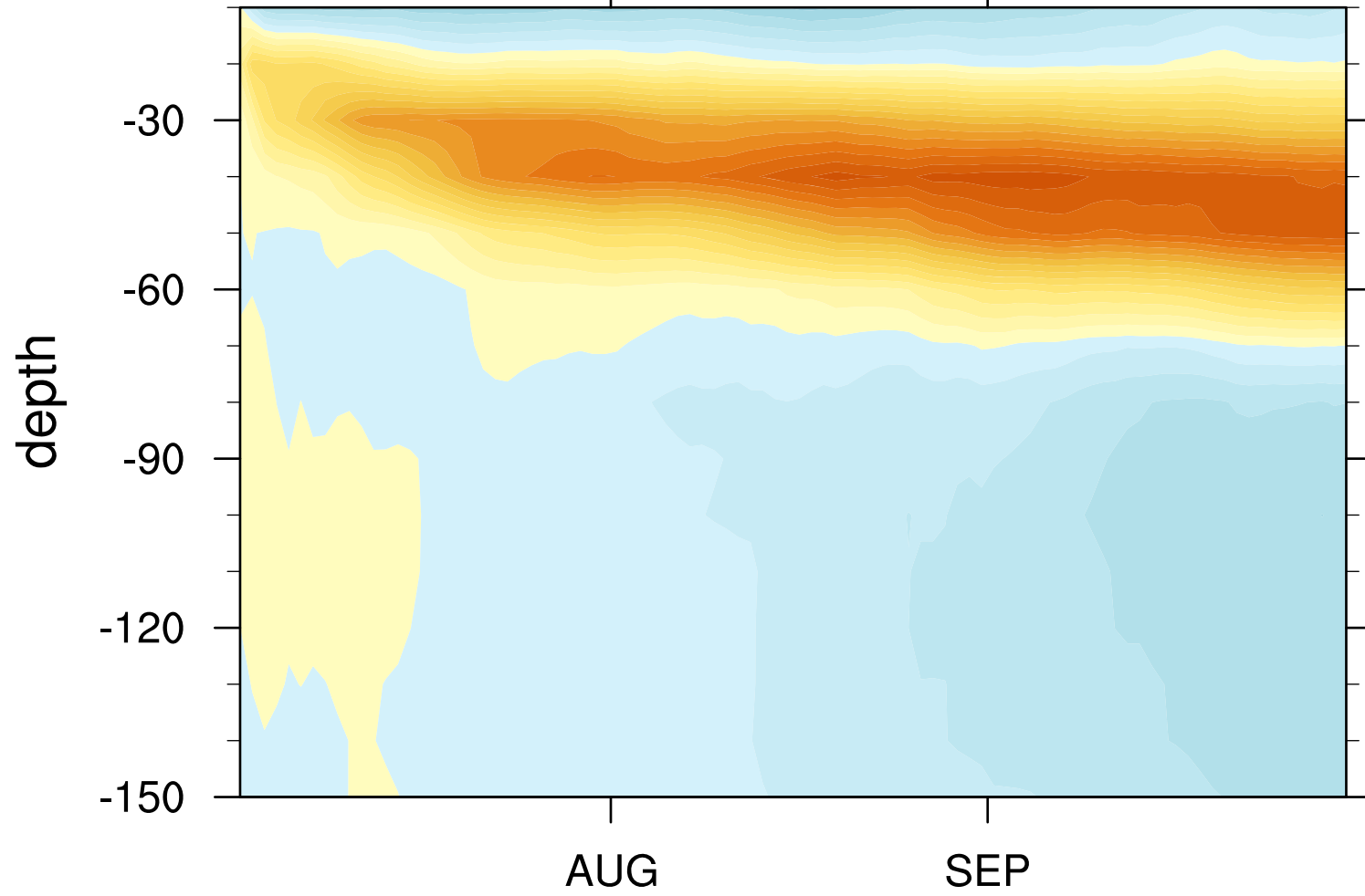
(b) Y21_RP - Y21_VT SALT (psu)
