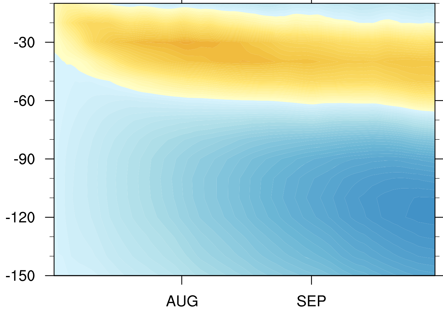
(a) Y21_RP - Y21_VT TEMP ( ^{\circ}\text{C} )
