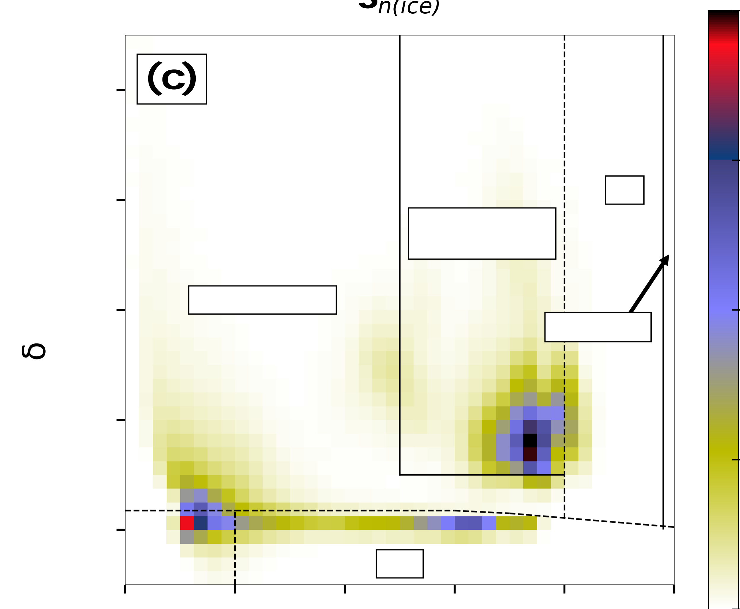
S_{n(ice)}
