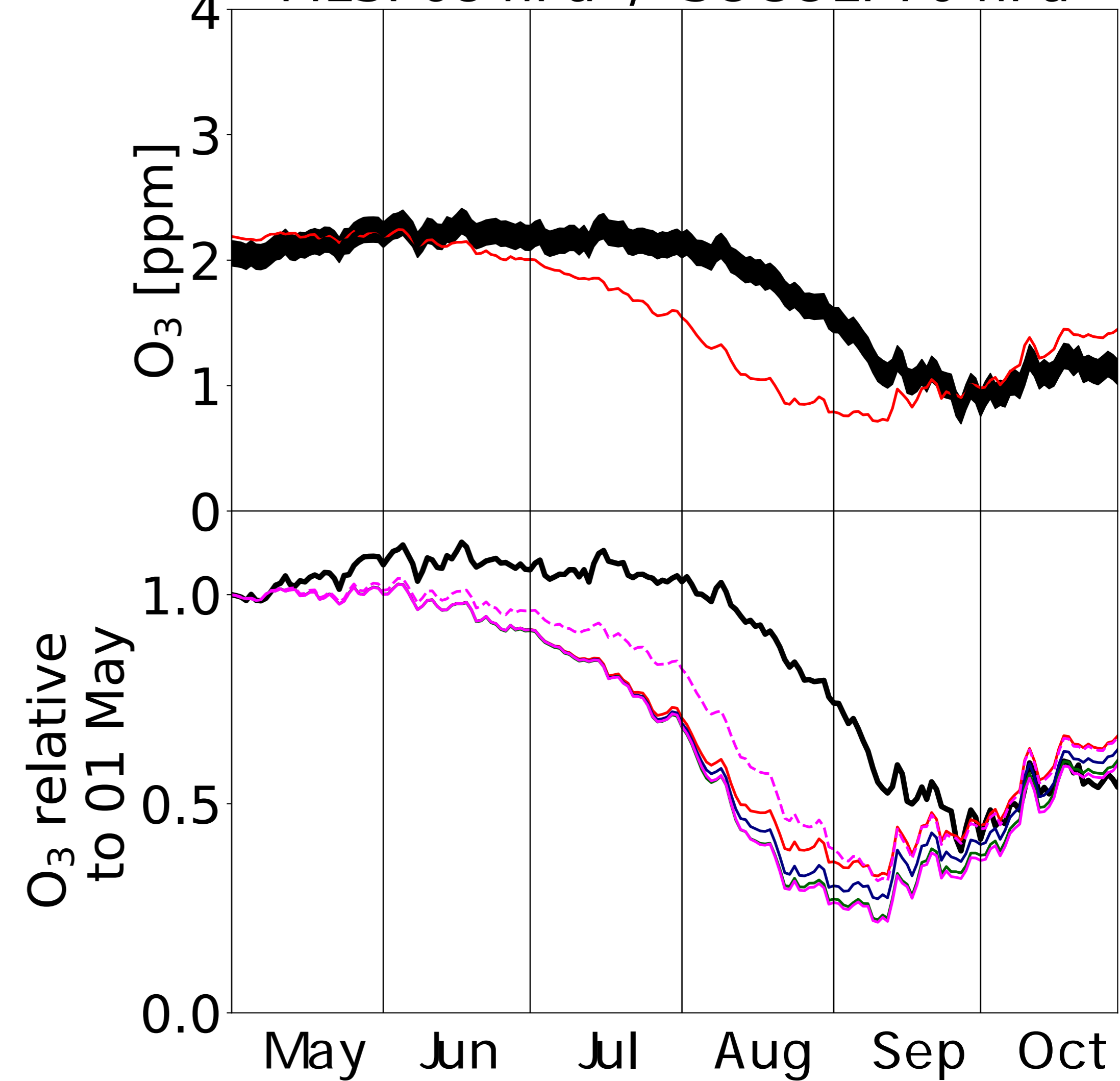
MLS: 68 hPa / SOCOL: 70 hPa
