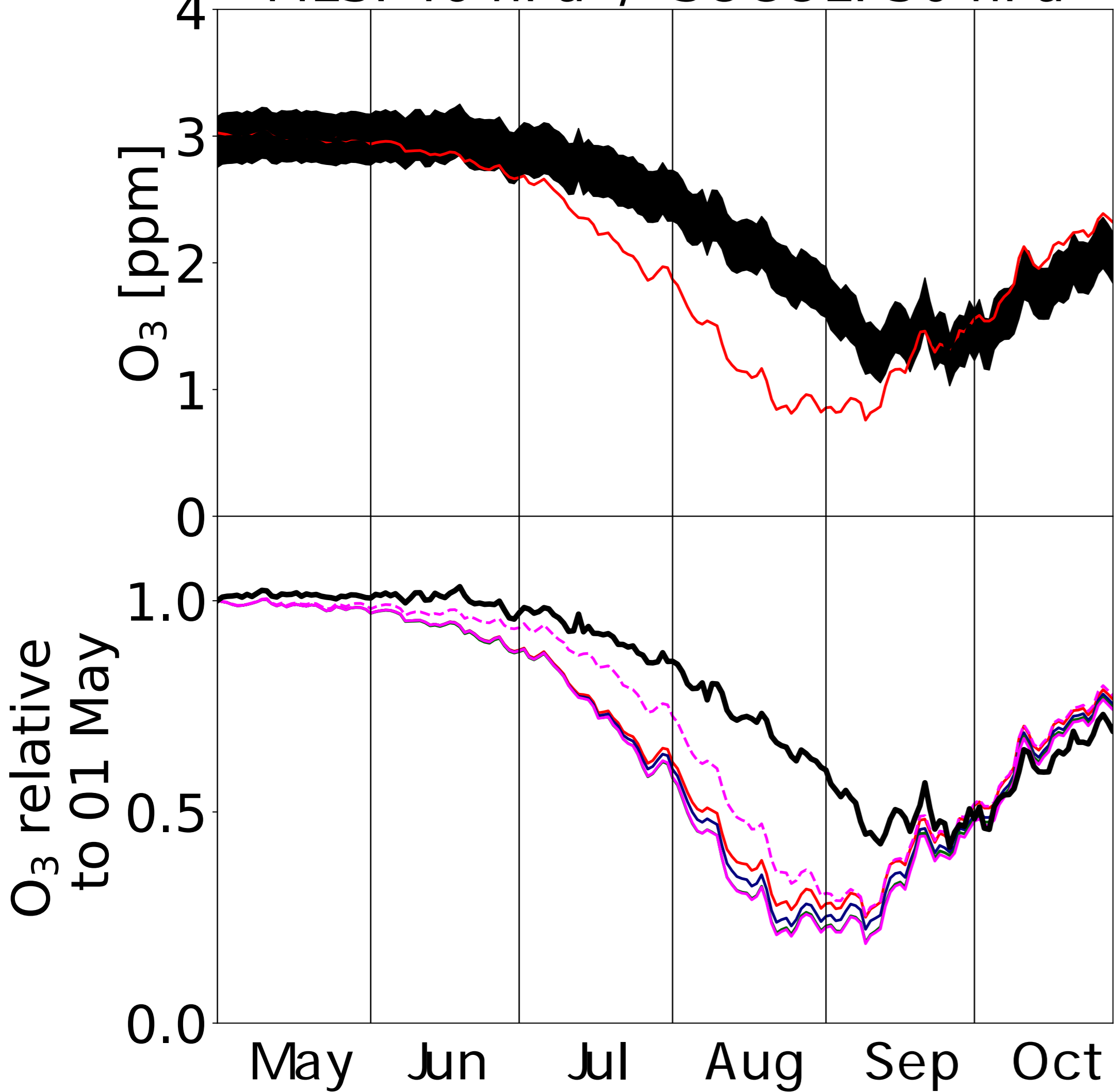
MLS: 46 hPa / SOCOL: 50 hPa
