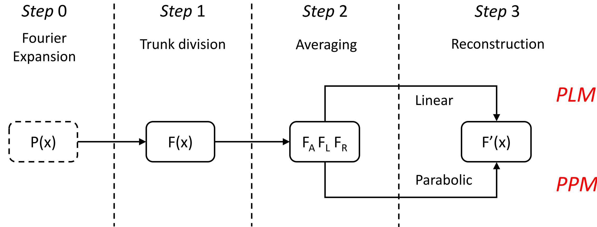
RING-AVERAGE ALGORITHM
